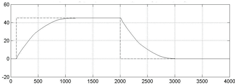
Fig. 5. Ship heading (solid) and desired ship heading (dashed)
