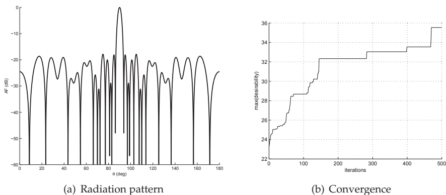
Fig. 5. Normalized radiation pattern and convergence of 32-element linear array obtained by the ant algorithm. ( SLL < -15 dB, BW < 7.7^\circ , and a null at 81^\circ )
