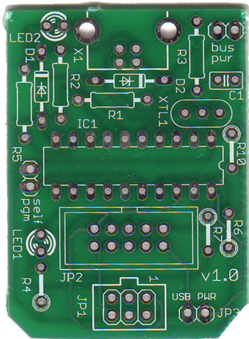
PCB Circuit board
