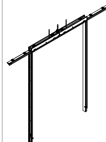
Portrait Double Barn Door Rail Kit for Full-Height Door – Low Profile (FPVGFR) and Portrait Double Barn Door Jamb Kit for Full-Height Glass Door – Low Profile (FPVGFJ)
