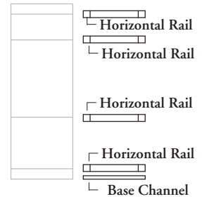
Working Wall Fascia Package (FPKHW)
