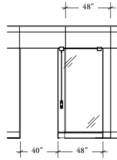
48" wide: 40" door clearance
