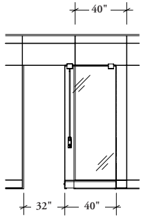
40" wide: 32" door clearance
