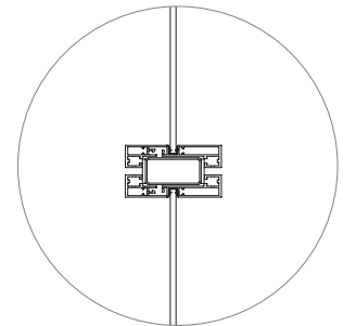
Section of square profile glass fascia
