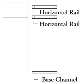
Full Fascia Package (FPKHF)
