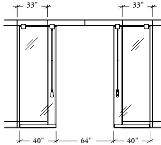
40" wide: 64" door clearance
