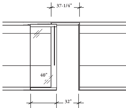
40" wide: 32" door clearance
