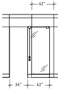
42" wide: 34" door clearance
