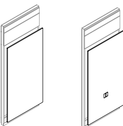
F P W 2 Solid Fascia – Working Wall (Level II)
