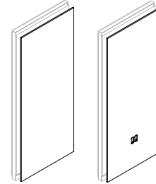
F P S 2 Solid Fascia – Segmented (Level II)
