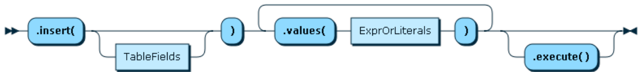
Figure 11.17 TableInsertFunction
