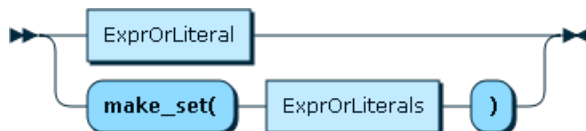
Figure 11.31 ExprOrLiteralOrOperand
