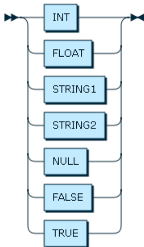
Figure 12.15 literal
