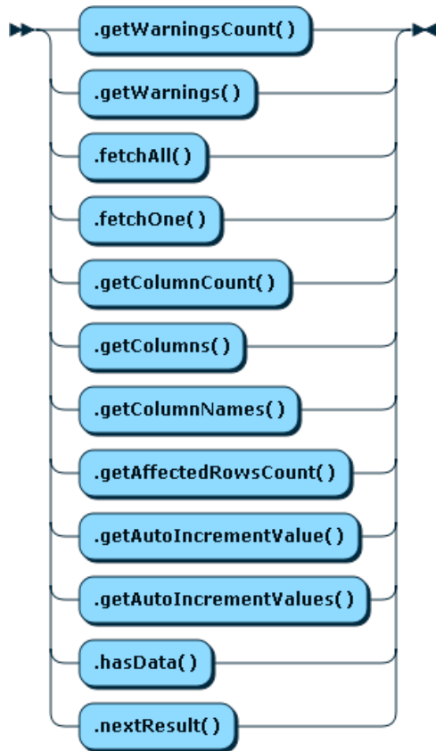
Figure 11.24 SqlResult
