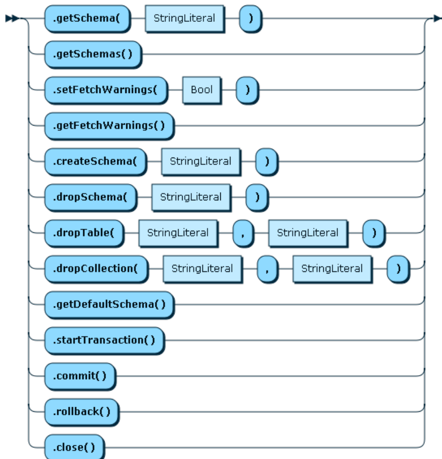
Figure 11.1 XSession
