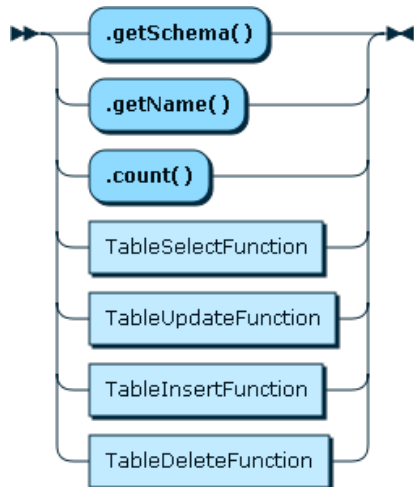
Figure 11.9 Table
