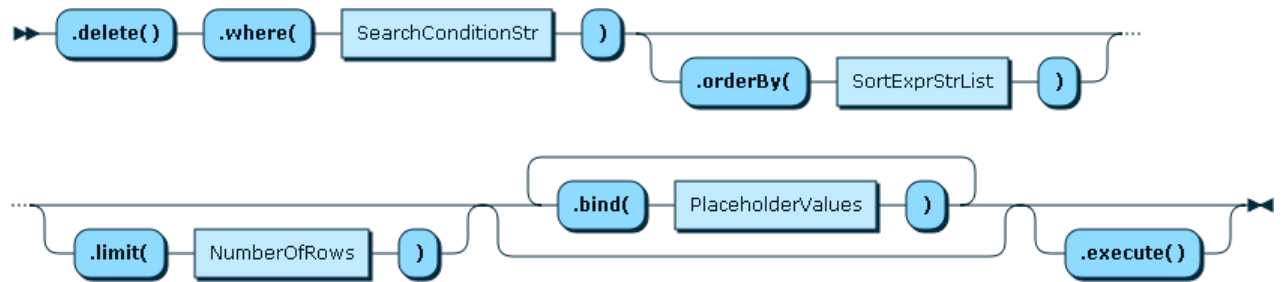
Figure 11.19 TableDeleteFunction
