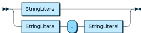
Figure 11.42 FunctionName
