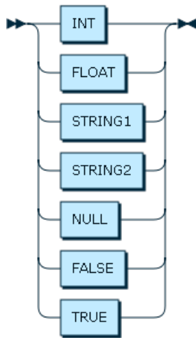
Figure 11.37 Literal
