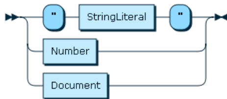
Figure 11.6 SQLLiteral
