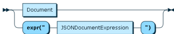
Figure 11.43 DocumentOrJSON
