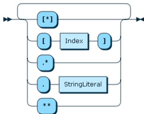
Figure 11.36 DocPath
