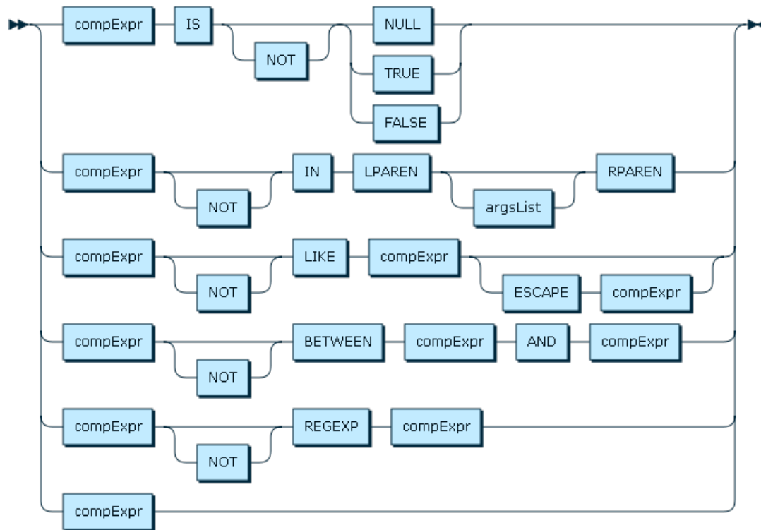
Figure 12.28 ilriExpr
