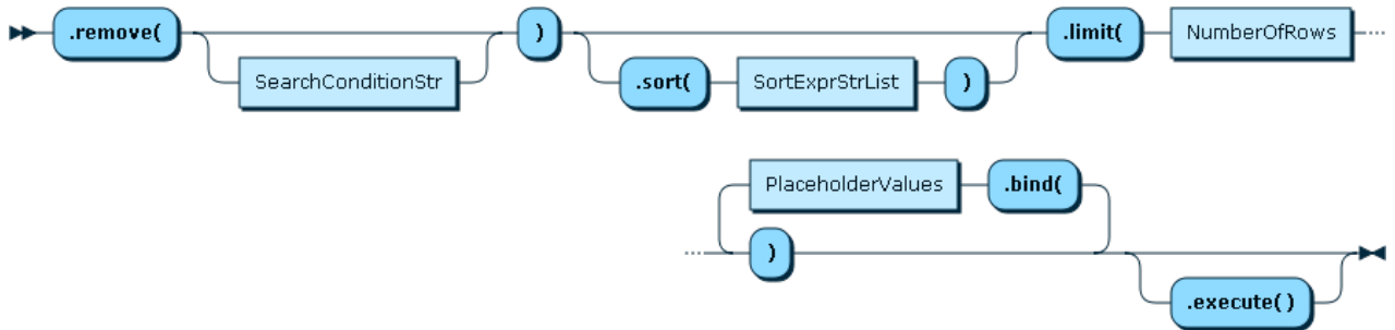
Figure 11.13 CollectionRemoveFunction
