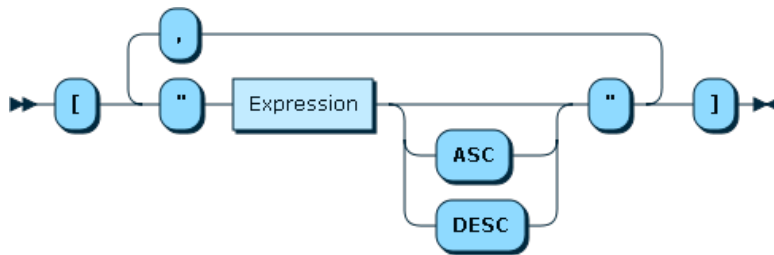
Figure 11.28 SortExprStrList
