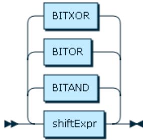
Figure 12.26 bitExpr
