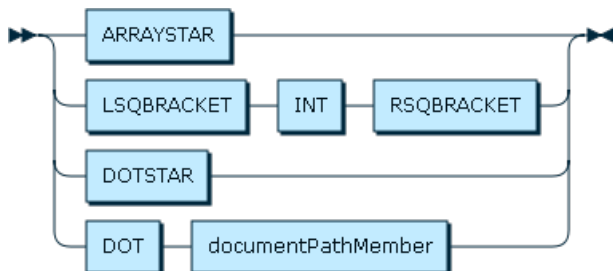
Figure 12.4 documentPathLastItem
