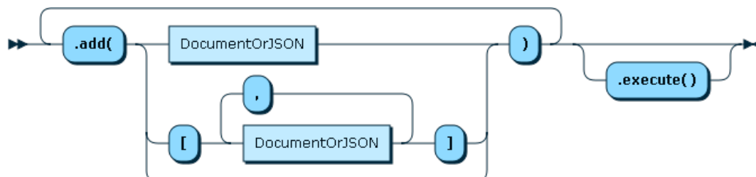
Figure 11.12 CollectionAddFunction
