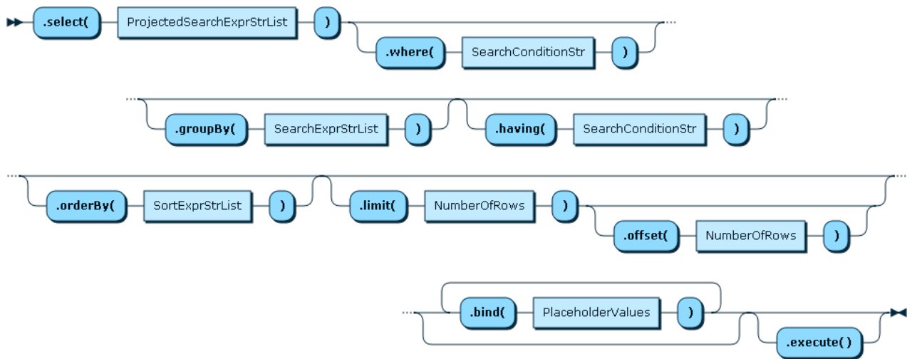
Figure 11.16 TableSelectFunction
