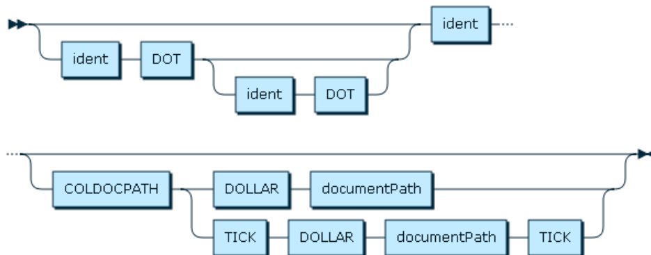
Figure 12.3 columnIdent
