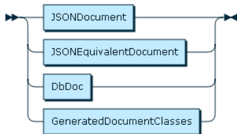
Figure 11.39 Document
