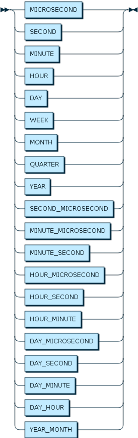
Figure 12.20 intervalUnit
