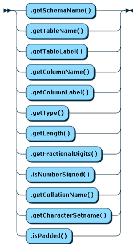
Figure 11.23 Column
