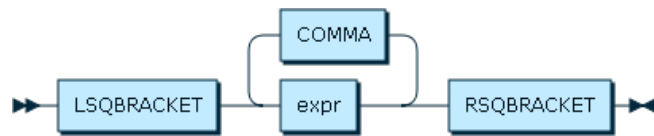
Figure 12.18 array
