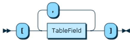
Figure 11.46 TableFields
