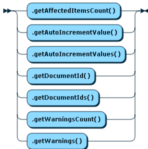
Figure 11.20 Result
