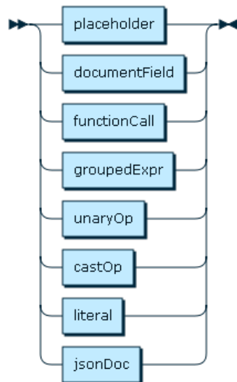
Figure 12.19 atomicExpr
