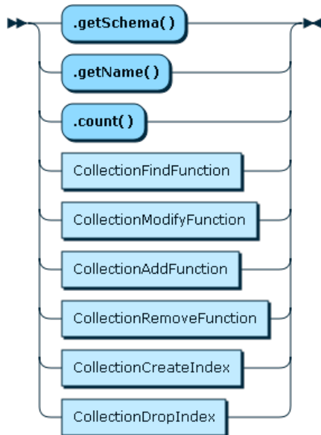
Figure 11.8 Collection
