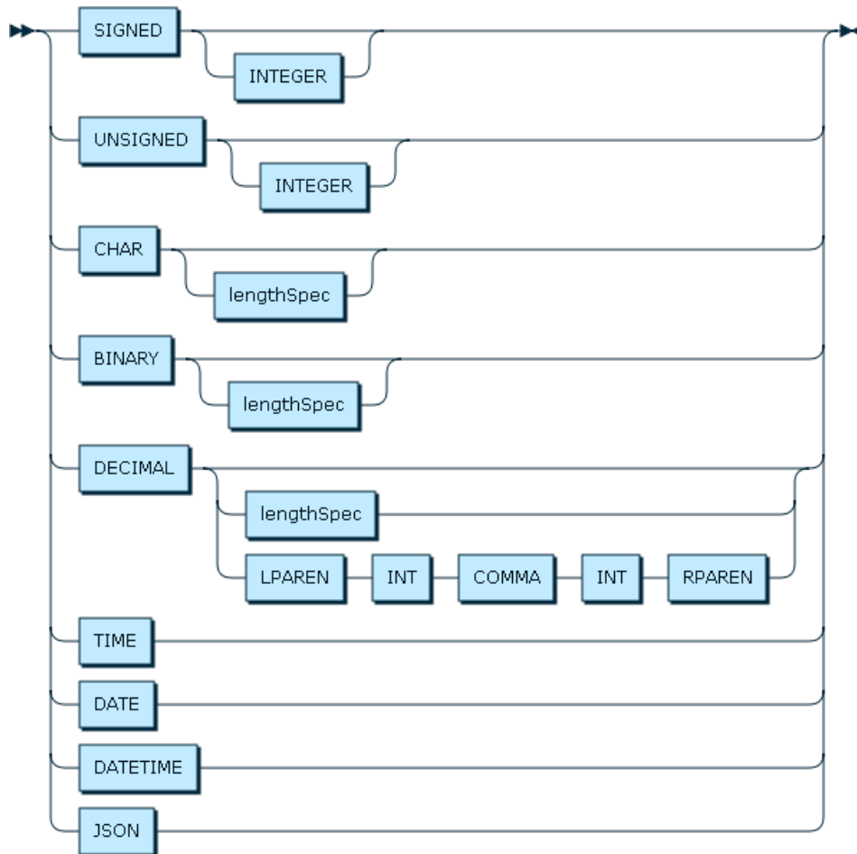
Figure 12.10 castType
