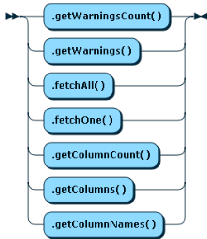
Figure 11.22 RowResult
