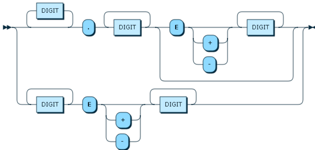
Figure 12.33 FLOAT
