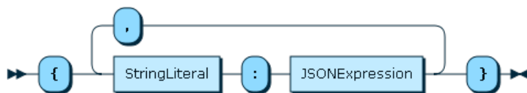
Figure 11.41 JSONDocumentExpression
