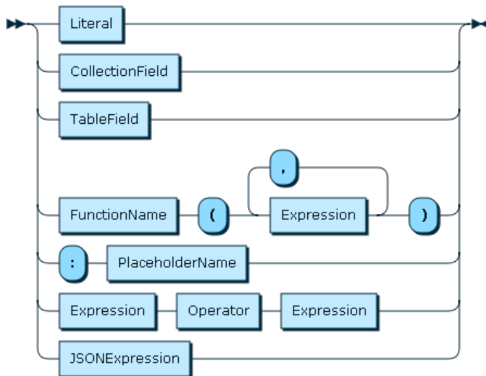
Figure 11.38 Expression
