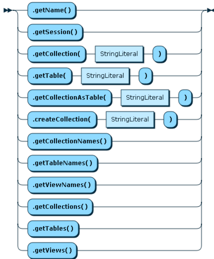
Figure 11.7 Schema
