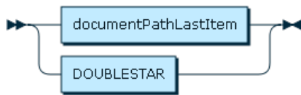
Figure 12.5 documentPathItem
