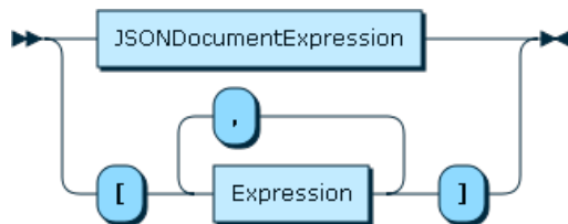
Figure 11.40 JSONExpression
