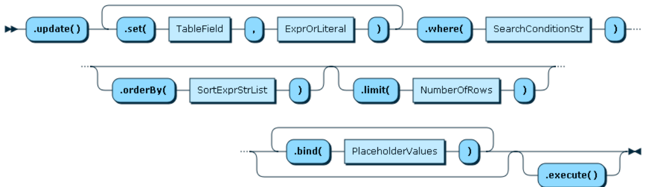
Figure 11.18 TableUpdateFunction
