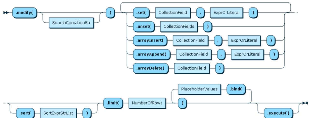
Figure 11.11 CollectionModifyFunction
