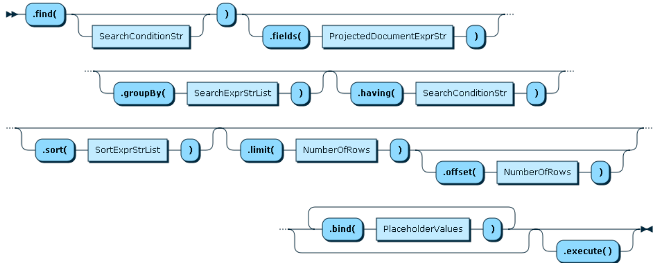
Figure 11.10 CollectionFindFunction
