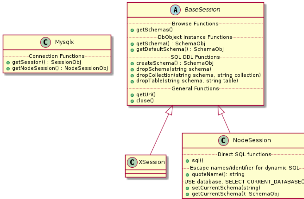
Figure 2.1 Session - Class Diagram
