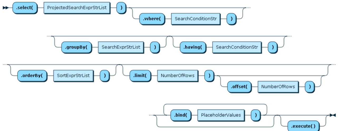
Figure 6.2 Table.select() Syntax Diagram
