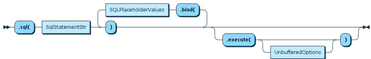
Figure 11.3 SqlExecute
