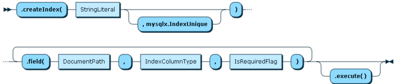
Figure 11.14 CollectionCreateIndex
