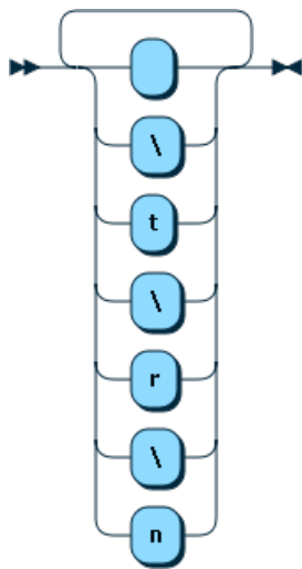
Figure 12.37 WS
