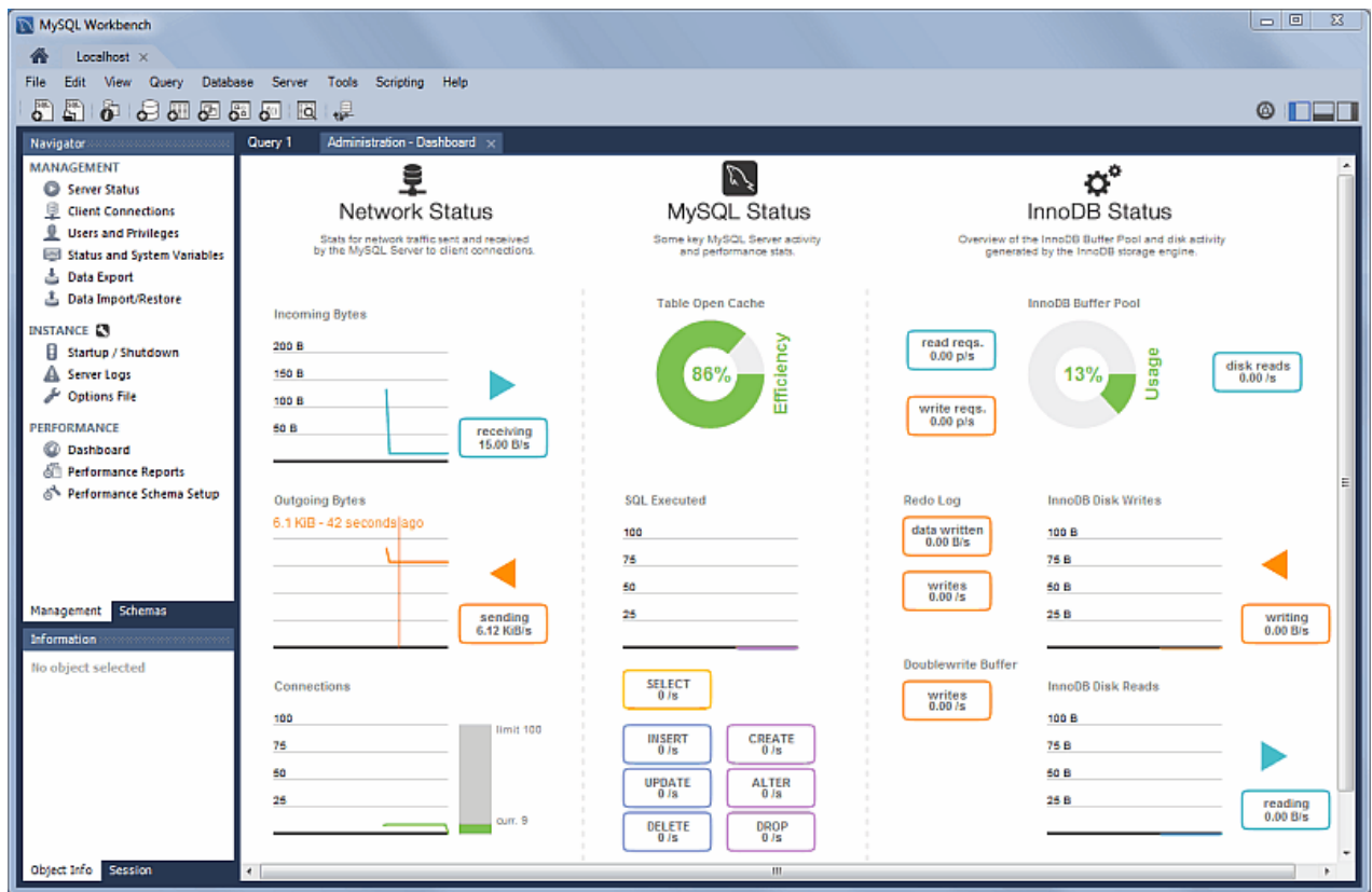
Figure 1.19 Performance Dashboard
