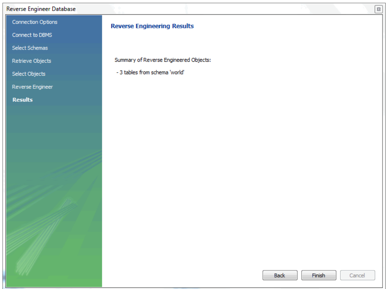
Figure 9.49 Results
