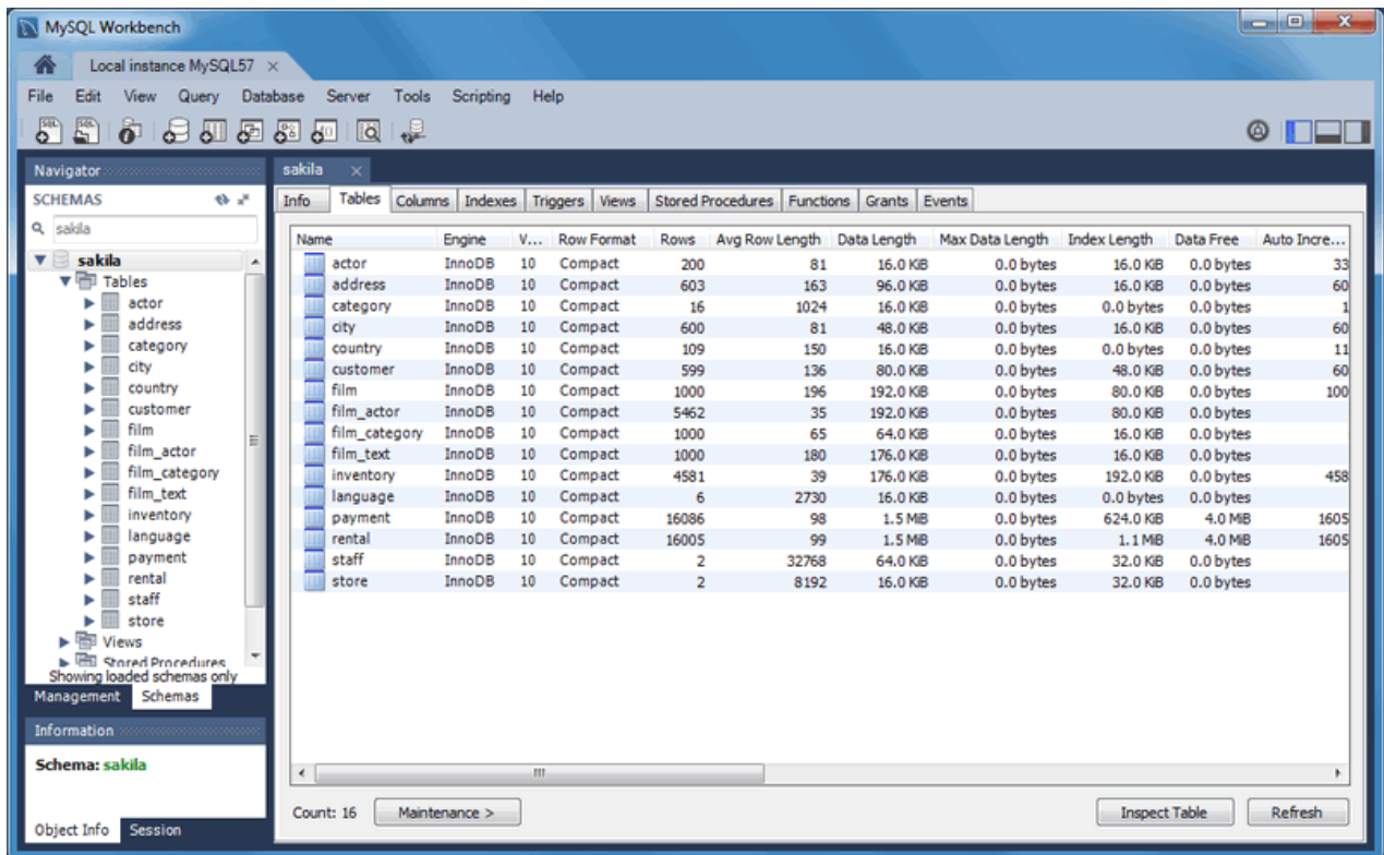
Figure 8.23 Schema Inspector
