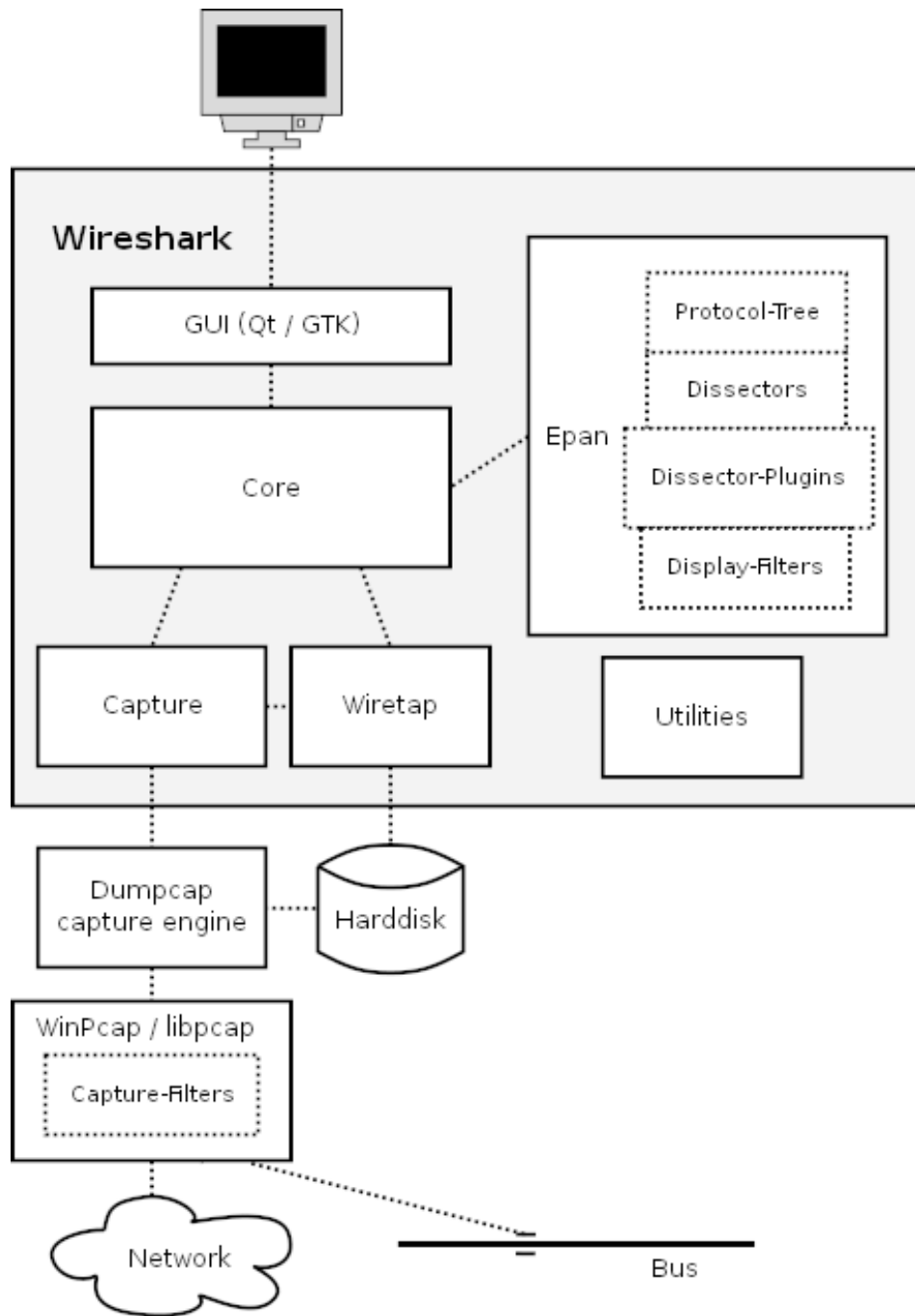
Figure 6.1. Wireshark function blocks
