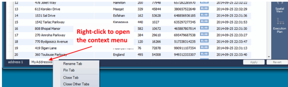
Figure 8.5 SQL Editor - Result Grid Context Menu
