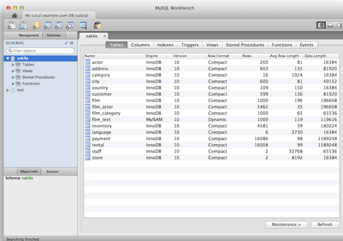
Figure 1.41 Schema Inspector
