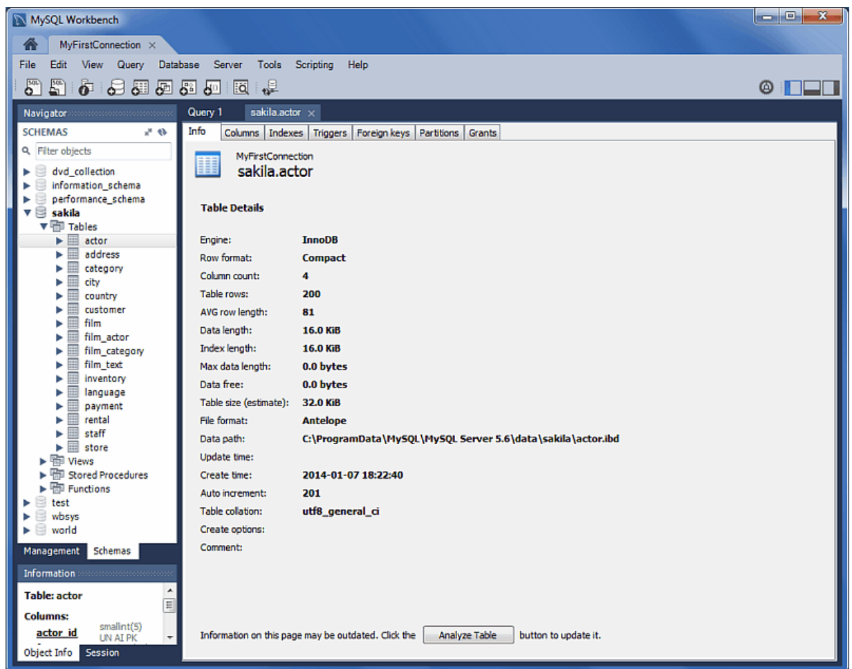
Figure 1.32 Table Inspector
