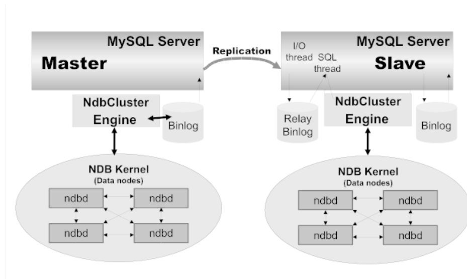
Figure 21.28 NDB Cluster -to-Cluster Replication Layout
