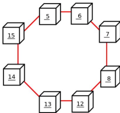
Figure 21.24 Circular Arrangement of NDB Cluster Nodes
