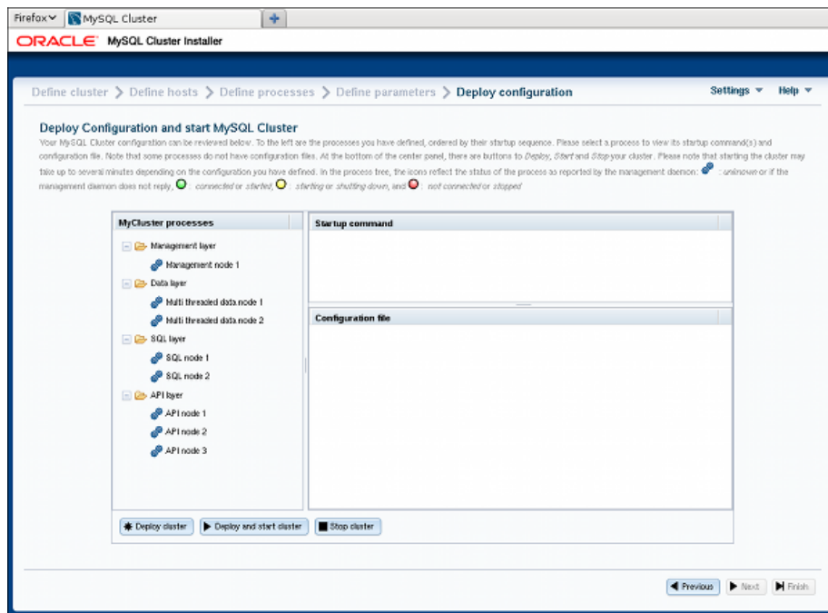
Figure 21.20 NDB Cluster Auto-Installer Deploy Cluster screen
