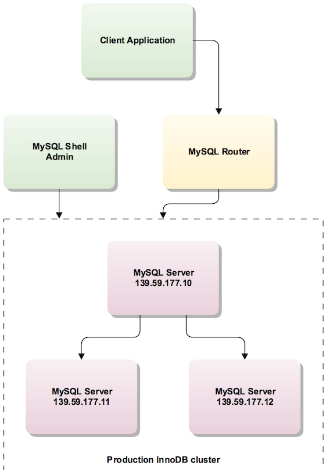
Figure 20.2 Production Deployment
