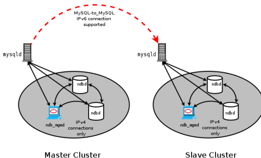
Figure 21.31 Replication Between SQL Nodes Connected Using IPv6
