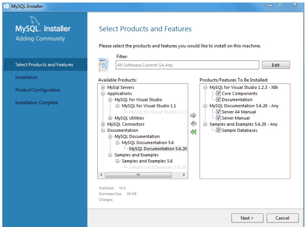
Figure 1.14 MySQL Installer - Select Products and Features
