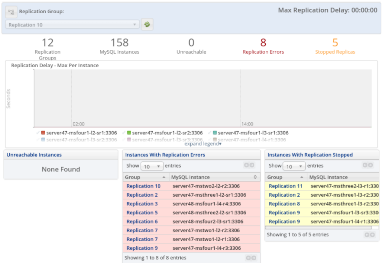
Figure 18.1 Replication Overview
