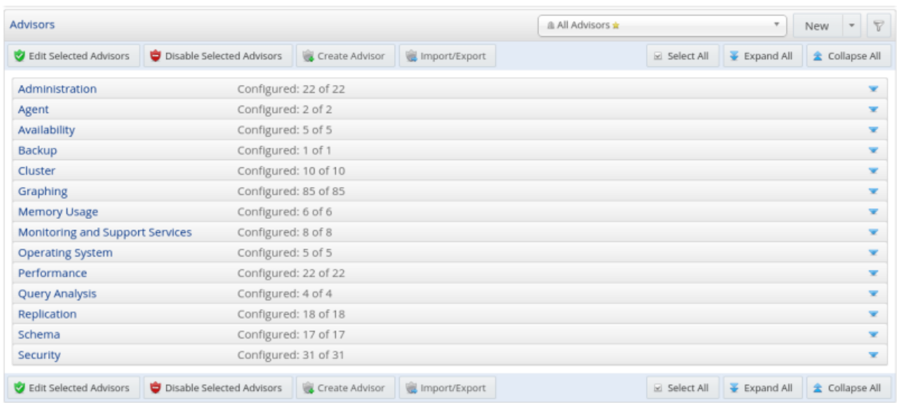
Figure 20.1 Advisors Page
