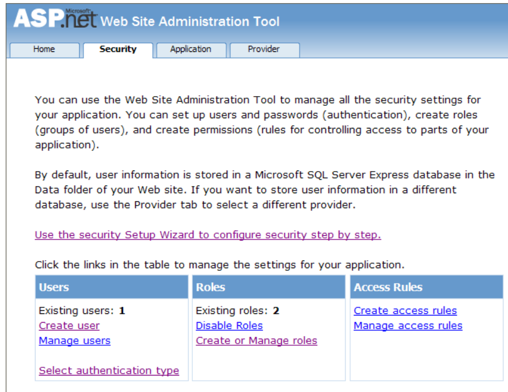
Figure 4.5 Security Tab
