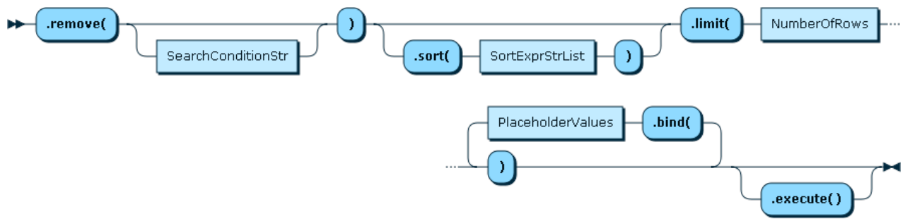
Figure 4.4 Collection.remove() Syntax Diagram
