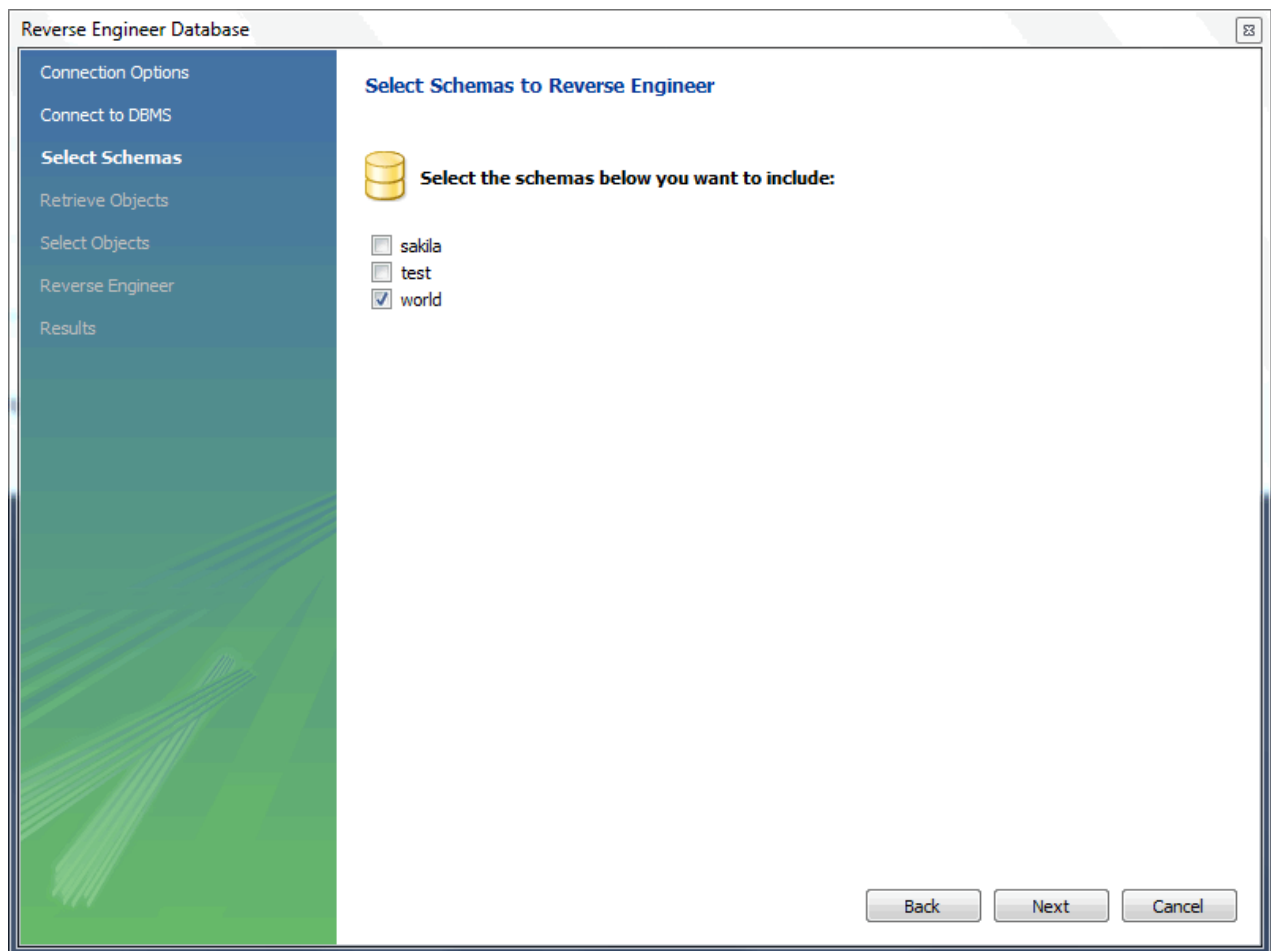
Figure 9.45 Select Schemas
