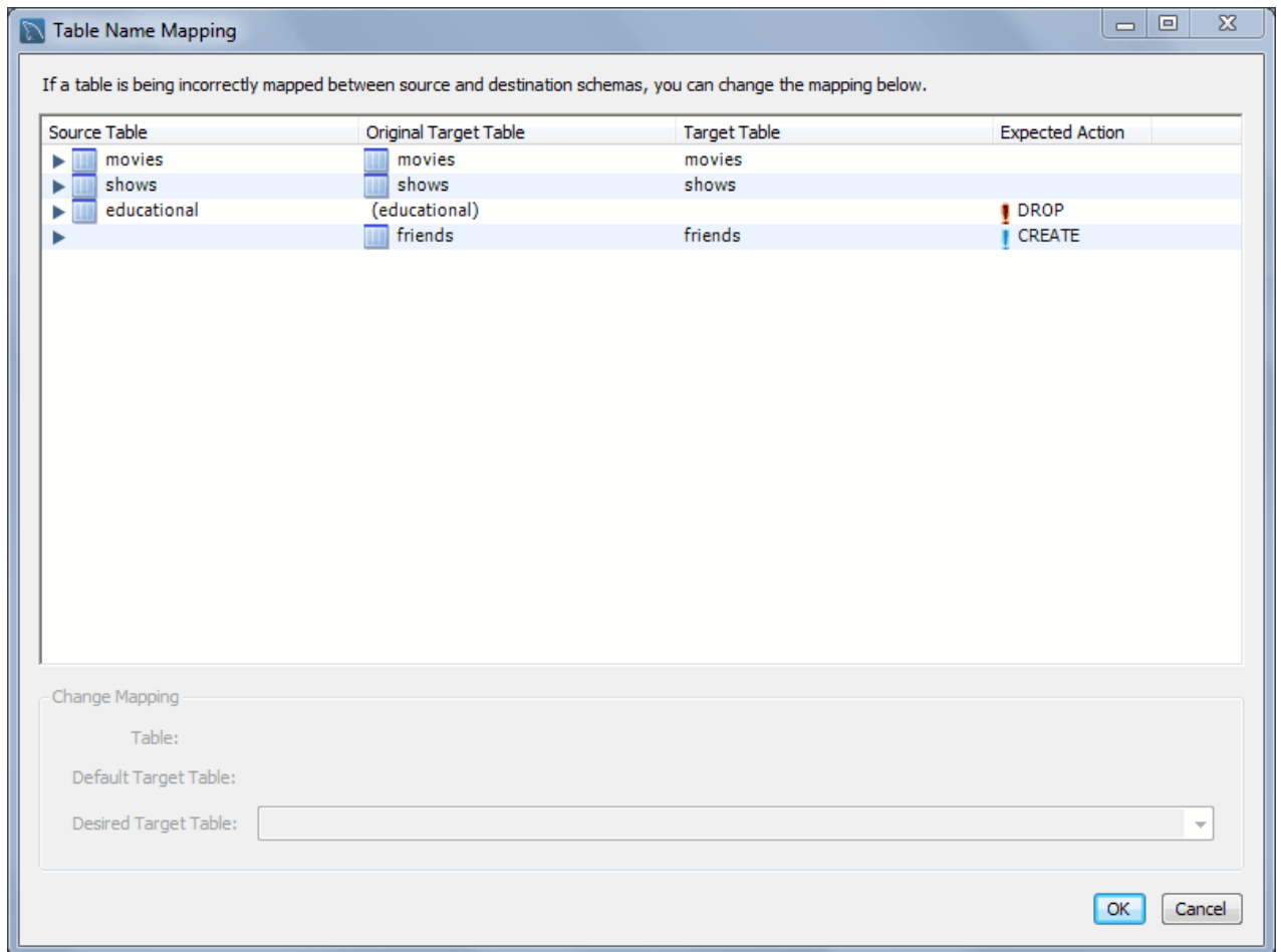
Figure 9.53 Table Mapping
