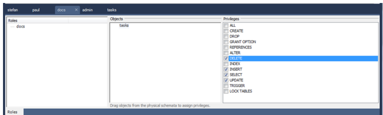
Figure 9.5 Role Editor
