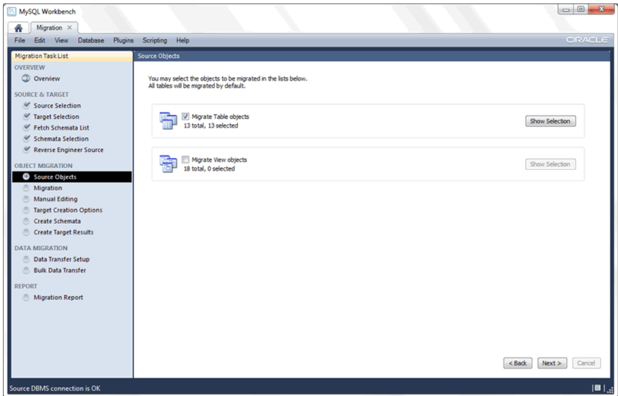
Figure 10.30 Source Objects
