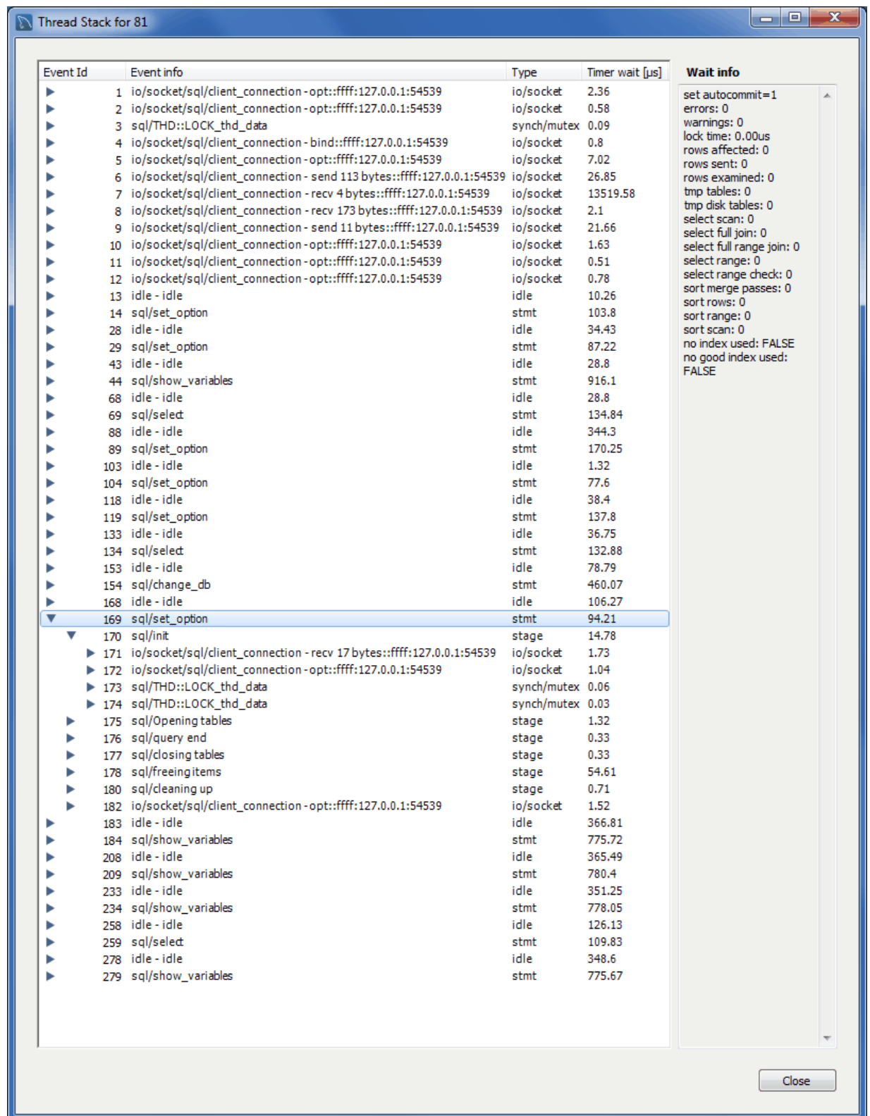
Figure 1.35 Client Connections: View Thread Stack
