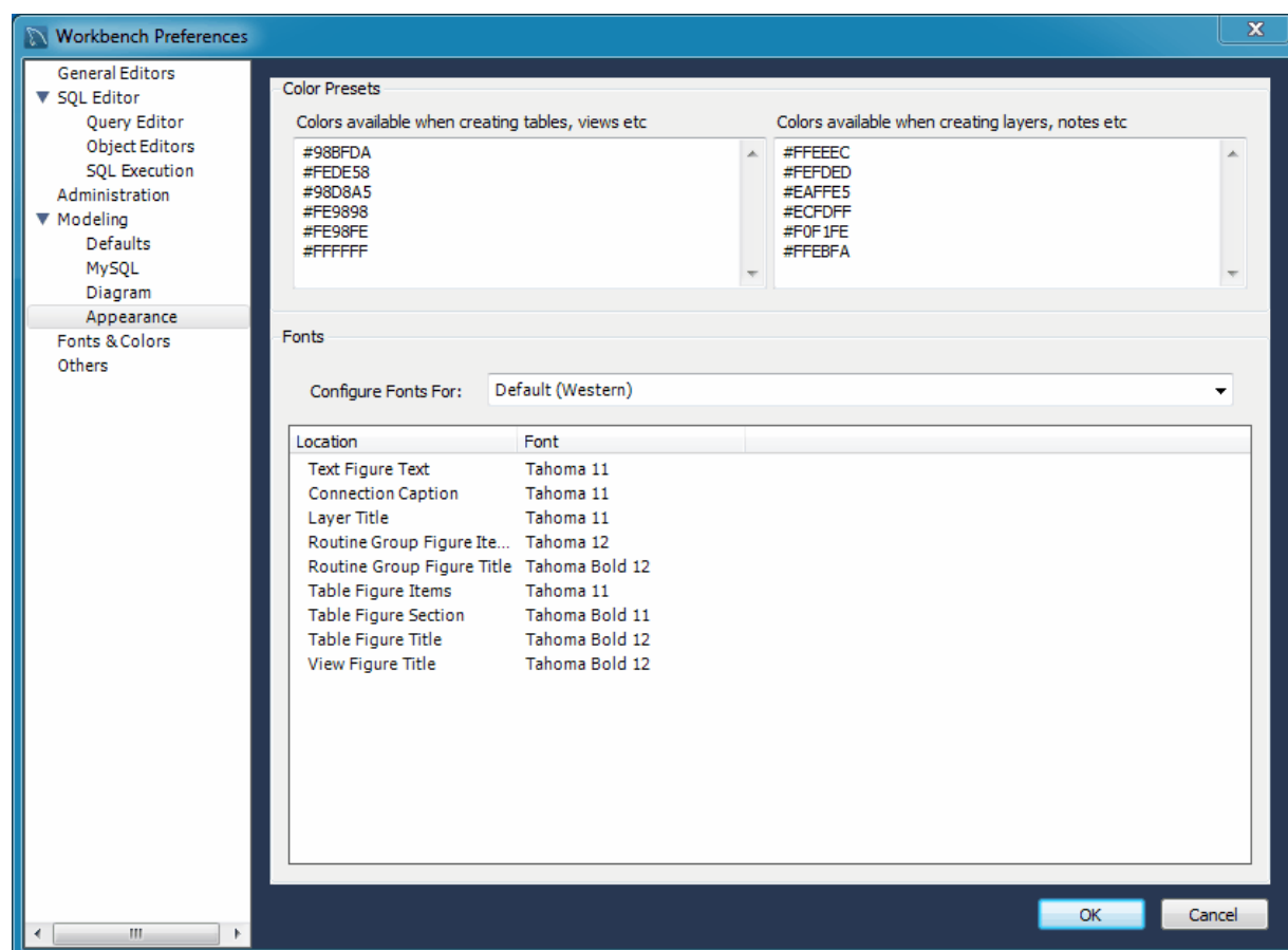
Figure 3.1 Appearance Preferences
