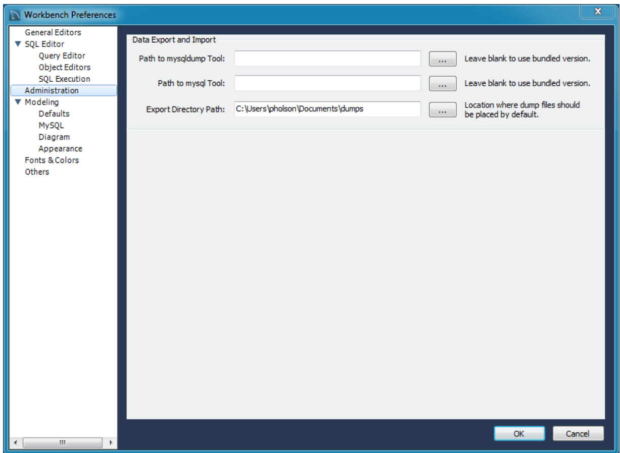
Figure 3.10 Preferences: Administration
