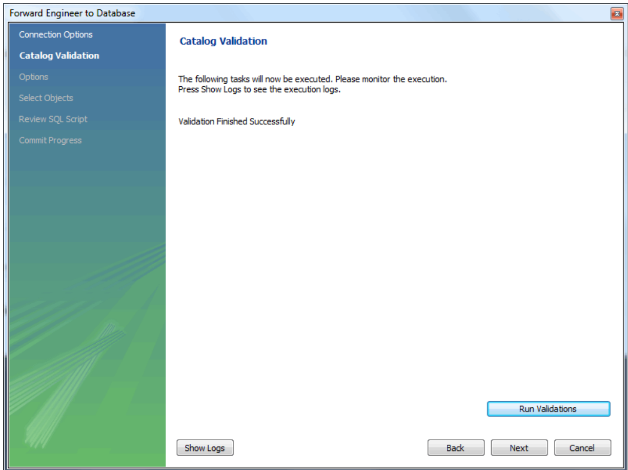
Figure 9.35 Catalog Validation
