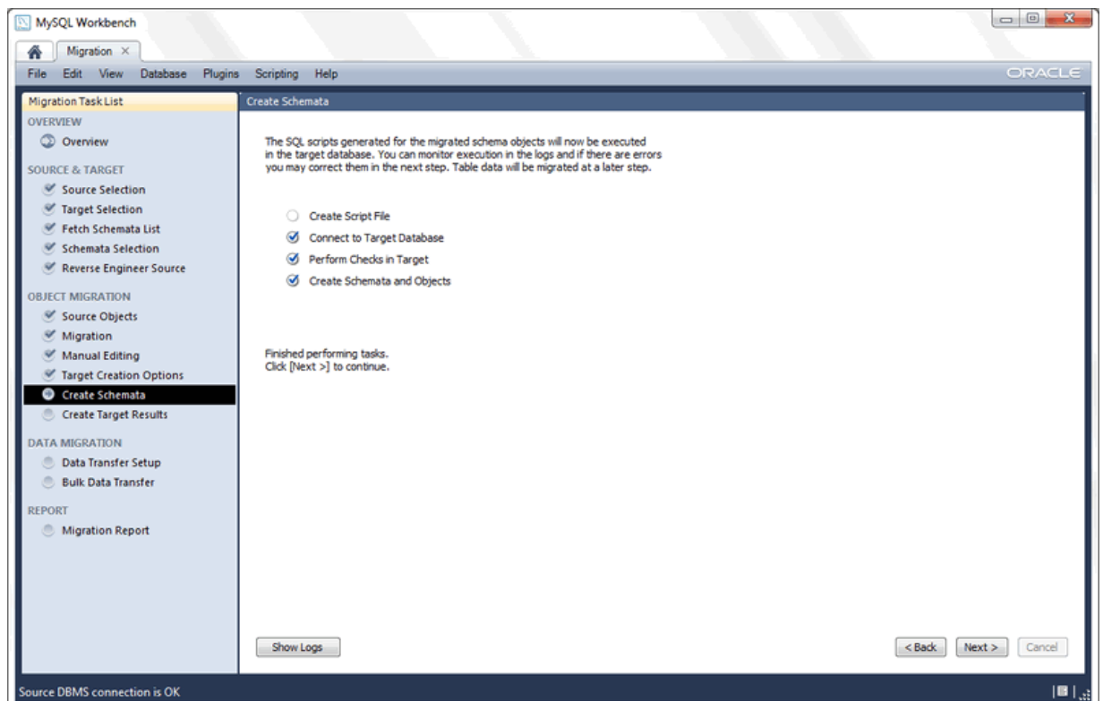
Figure 10.36 Create Schemata
