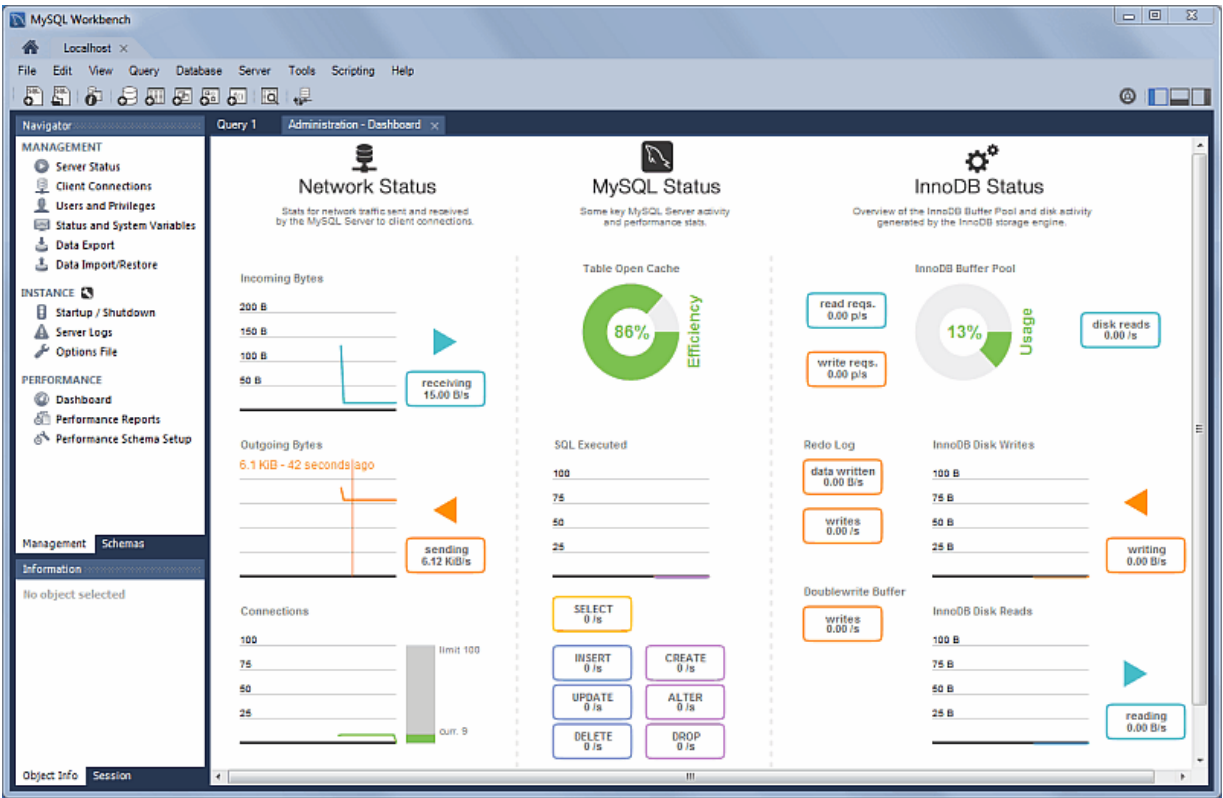
Figure 7.1 Performance: Dashboard
