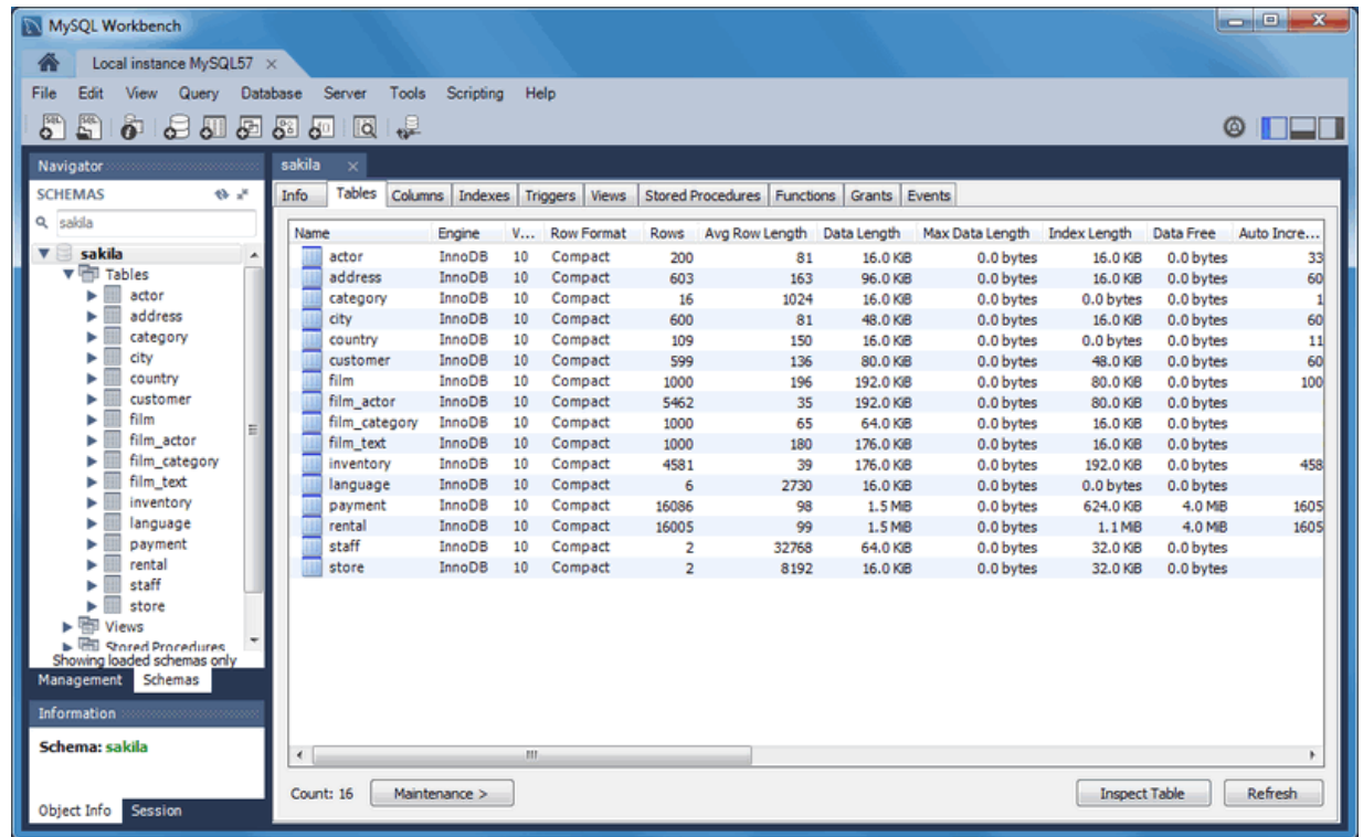
Figure 8.27 Schema Inspector
