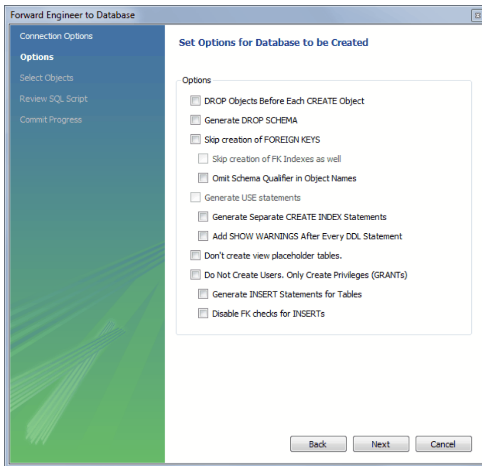
Figure 9.36 Options
