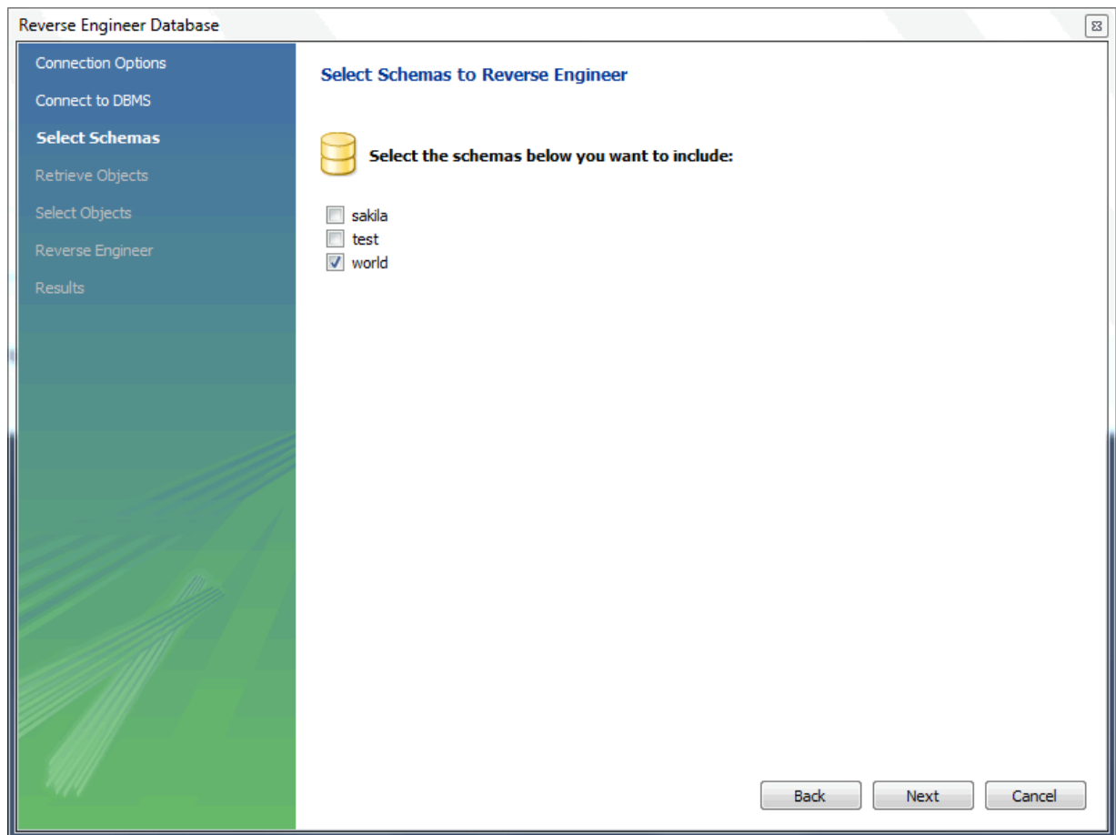
Figure 9.45 Select Schemas
