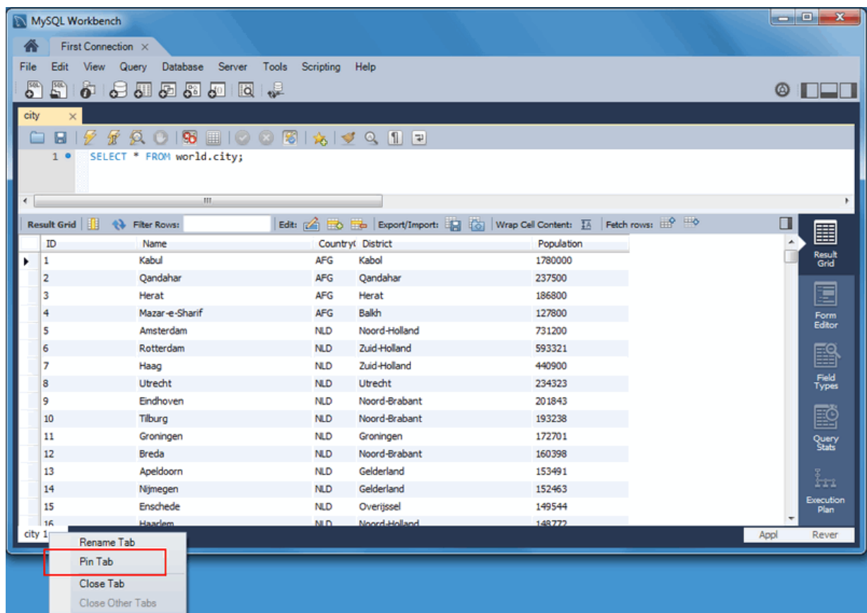
Figure 1.10 Pin Tab
