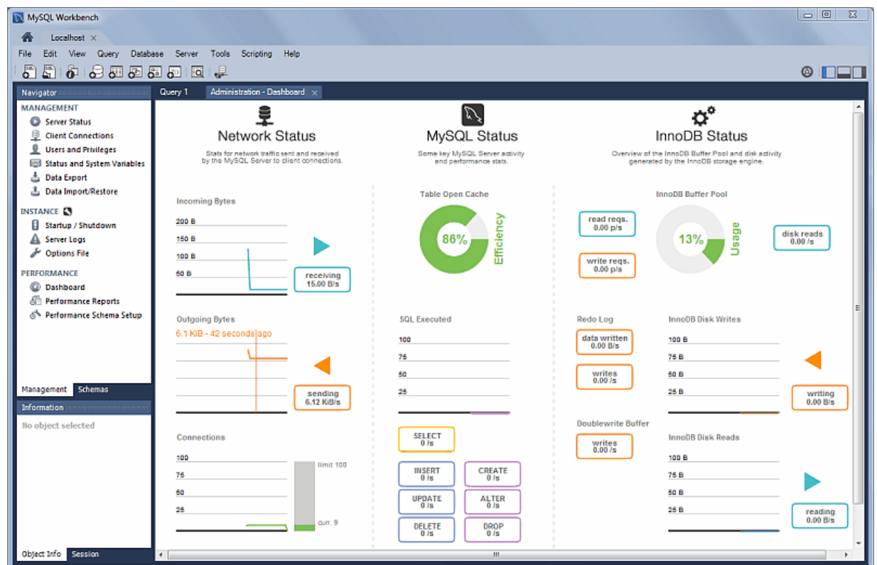
Figure 1.21 Performance Dashboard
