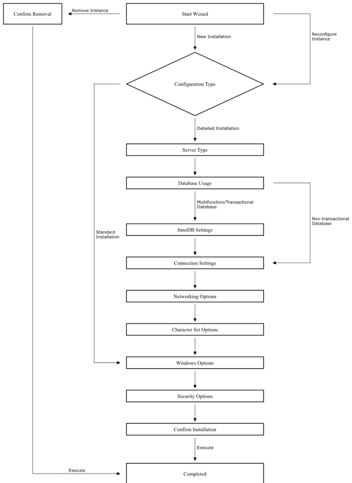
Figure 1.12 MySQL Server Instance Config Wizard Workflow
