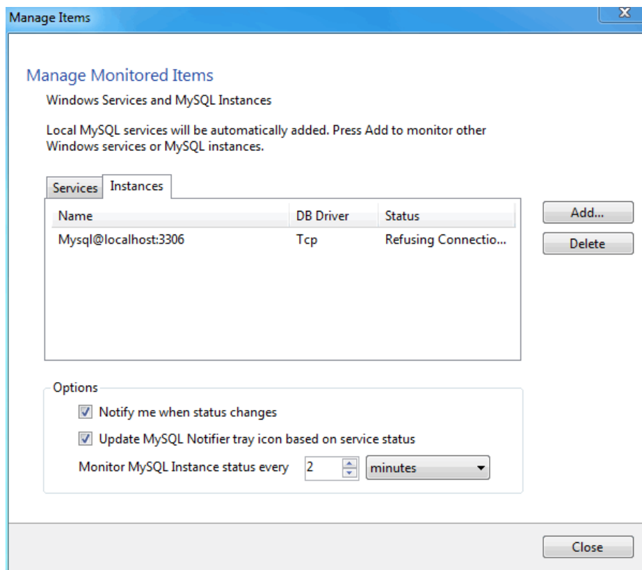
Figure 3.5 MySQL Notifier Manage Instances menu
