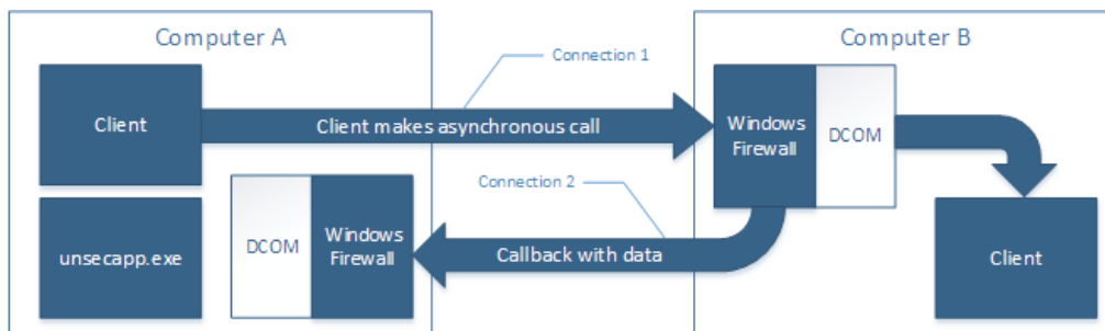
Figure 3.8 MySQL Notifier Distributed Component Object Model (DCOM)
