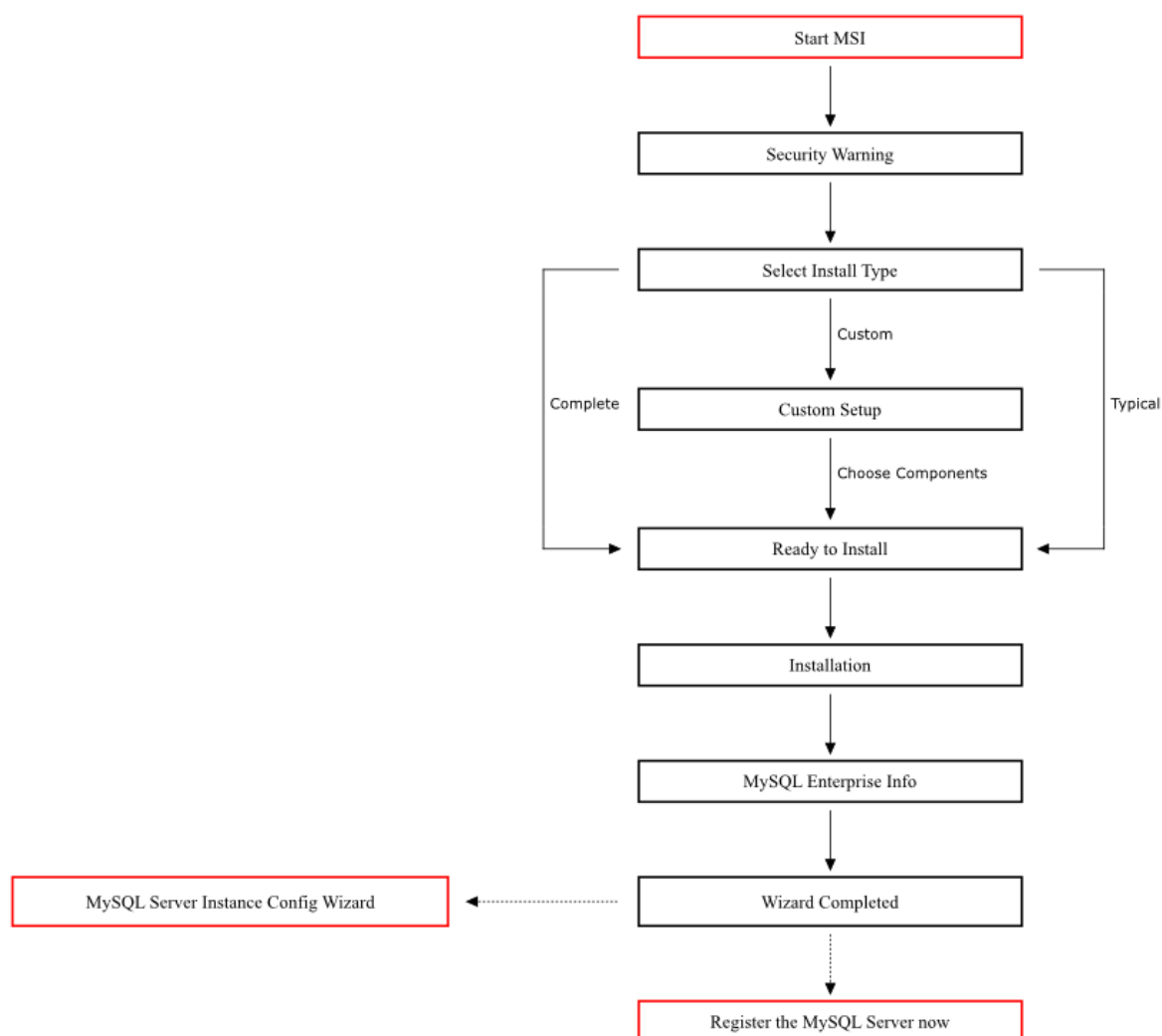
Figure 5.34 Installation Workflow for Windows Using MSI Installer
