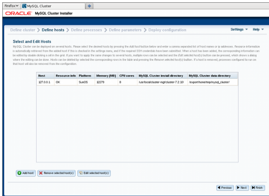
Figure 4.10 NDB Cluster Define Hosts screen
