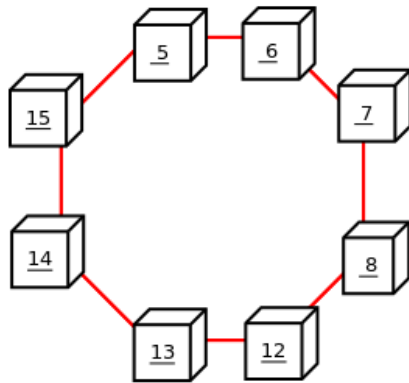
Figure 7.2 Circular Arrangement of NDB Cluster Nodes
