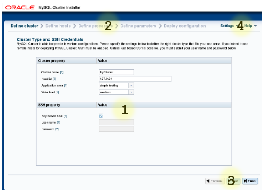
Figure 4.3 Layout of the NDB Cluster Auto-Installer GUI
