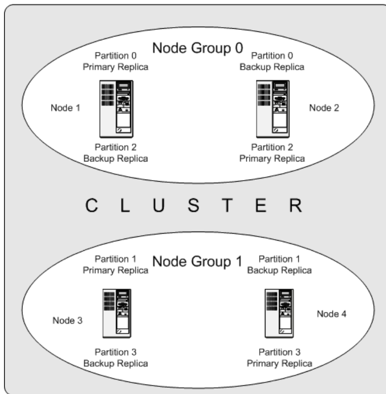
Figure 3.2 NDB Cluster with Two Node Groups
