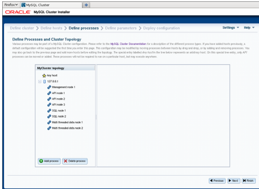
Figure 4.12 NDB Cluster Auto-Installer Define Processes dialog
