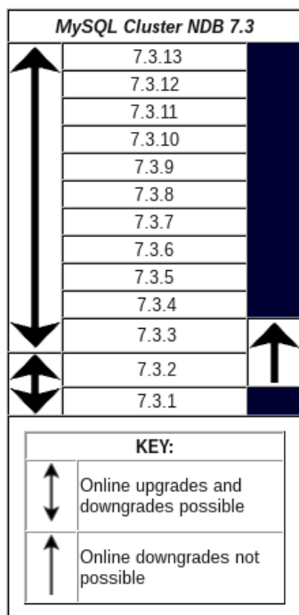
Figure 4.20 NDB Cluster Upgrade and Downgrade Compatibility, NDB Cluster 7.3
