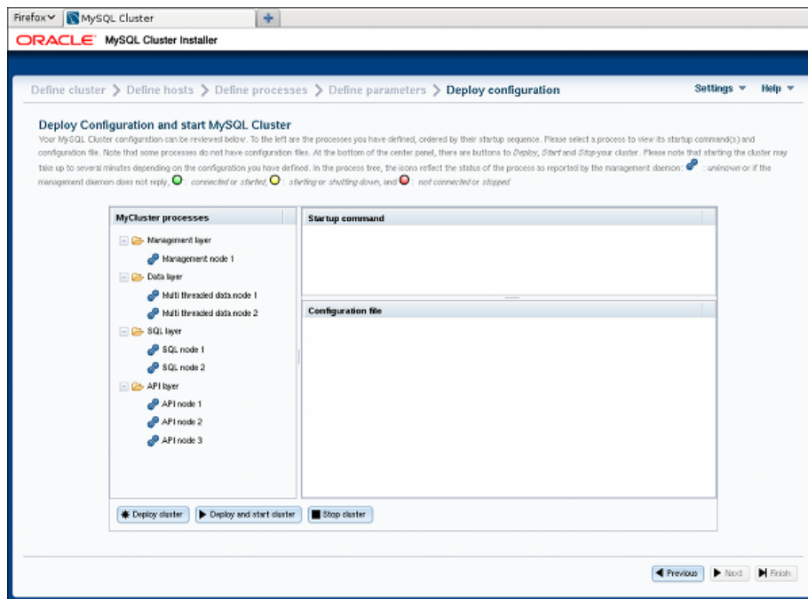
Figure 4.17 NDB Cluster Auto-Installer Deploy Cluster screen
