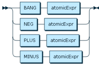
Figure 12.14 unaryOp
