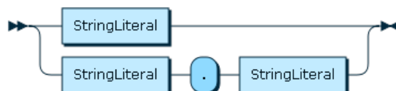
Figure 11.42 FunctionName
