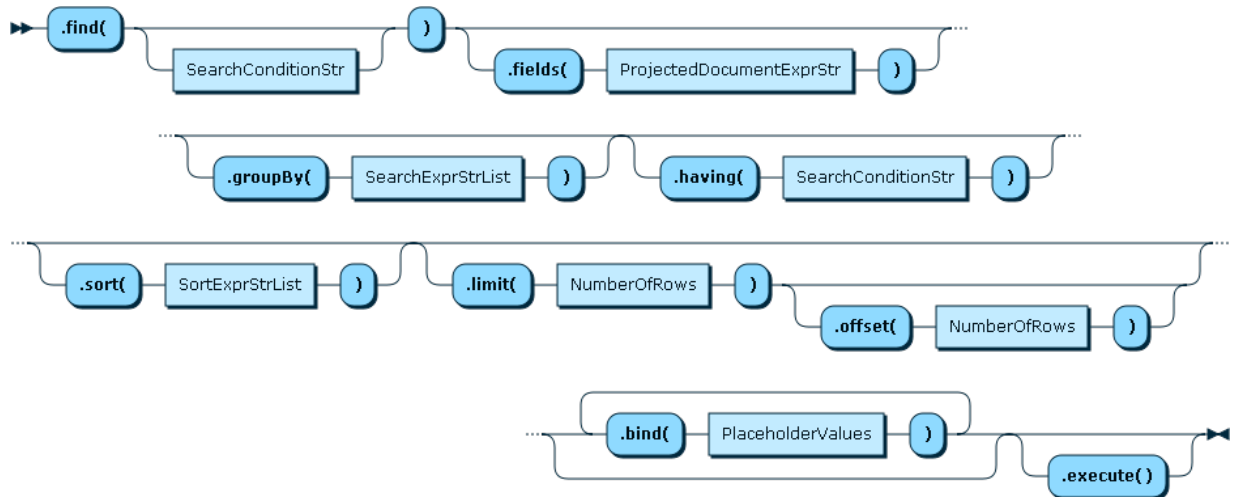
Figure 11.10 CollectionFindFunction
