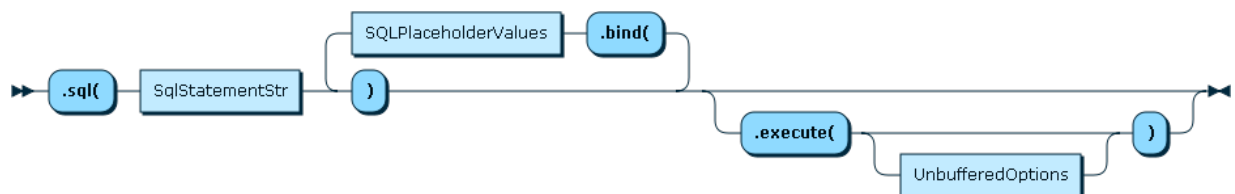
Figure 11.3 SqlExecute
