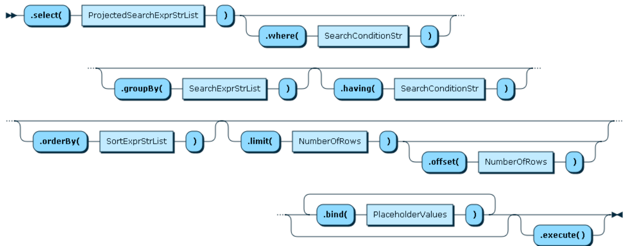
Figure 11.16 TableSelectFunction
