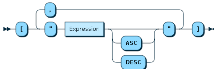
Figure 11.28 SortExprStrList
