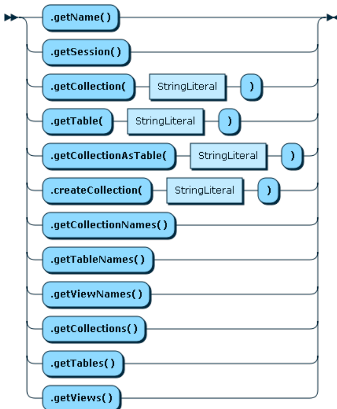
Figure 11.7 Schema
