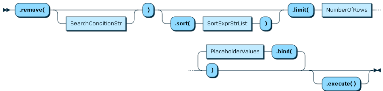
Figure 11.13 CollectionRemoveFunction
