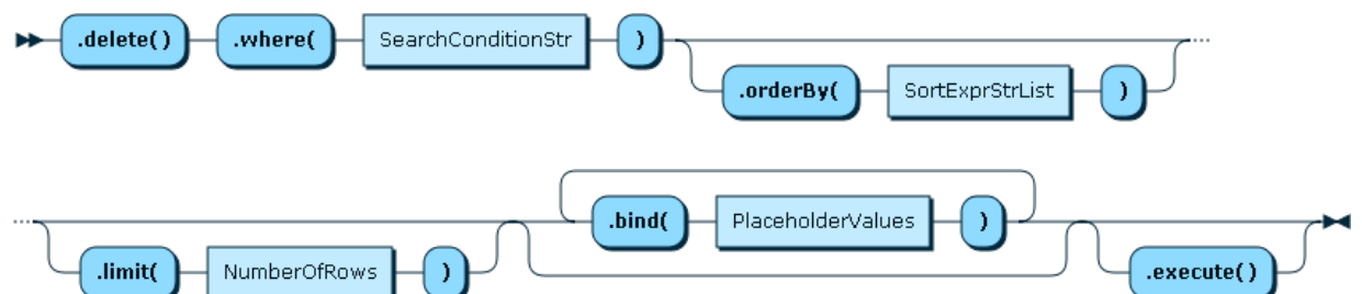
Figure 11.19 TableDeleteFunction
