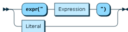
Figure 11.29 ExprOrLiteral
