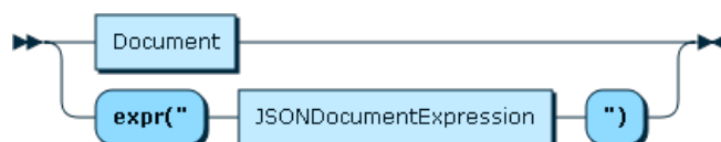
Figure 11.43 DocumentOrJSON
