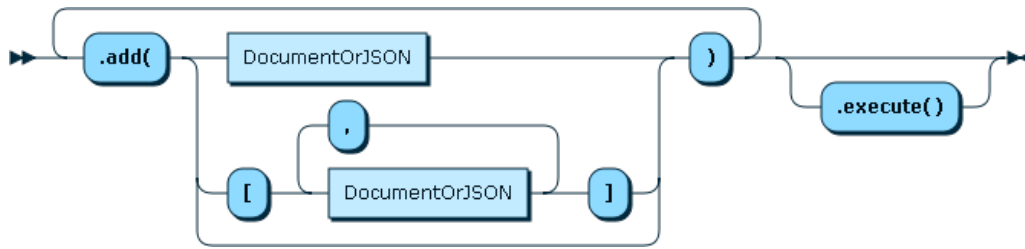
Figure 4.1 Collection.add() Syntax Diagram
