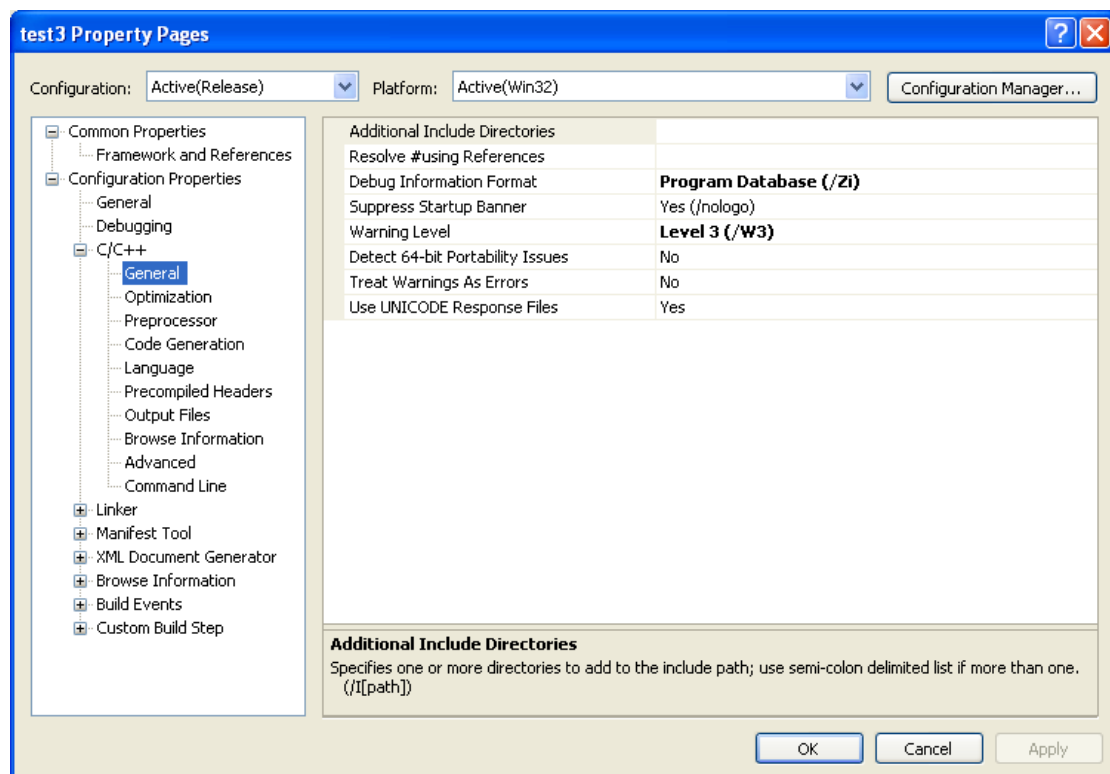
Figure 5.6 Setting Properties
