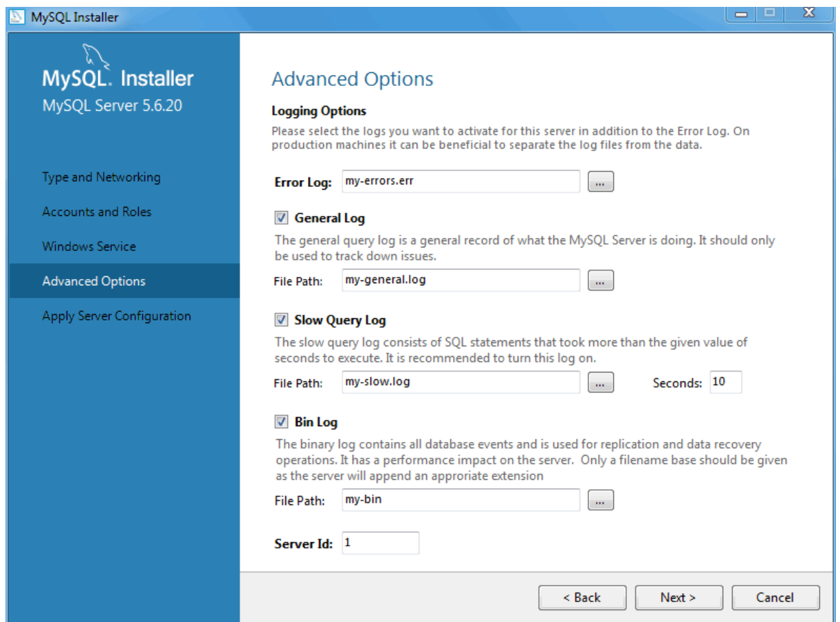
Figure 1.10 MySQL Installer - MySQL Server Configuration: Logging Options
