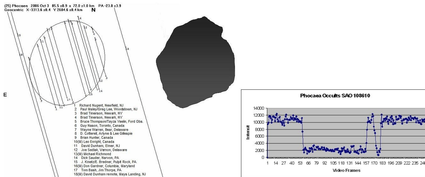
Figure 6.1a. Left - Profile of 25 Phocaea from occultation on October 3, 2006 using Occult software. Solid drawing is the derived line of sight shape of Phocaea from the observations drawn by Richard Nugent. Chords #3 and #4 are from Brad Timerson's video and show a valley or depression on the northwest side of the asteroid. Right-Limovie light curve shows Brad Timerson's double event from chord's #3 (3.4 second occultation) and #4 (0.30 second occultation).
