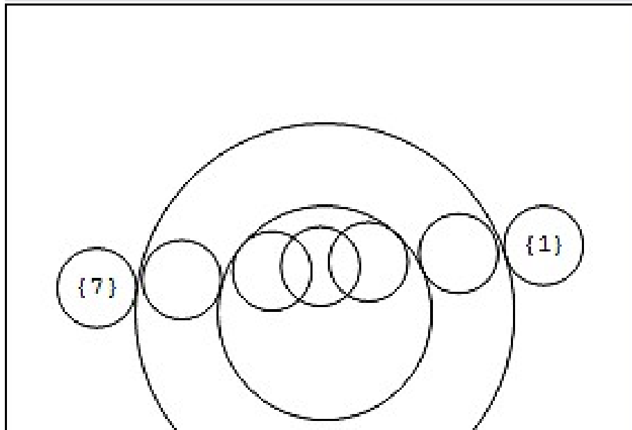
Figure 4.7. Lunar eclipse contact times. Earth orientations for each contact time and Moon's motion through Earth's shadow are displayed.
