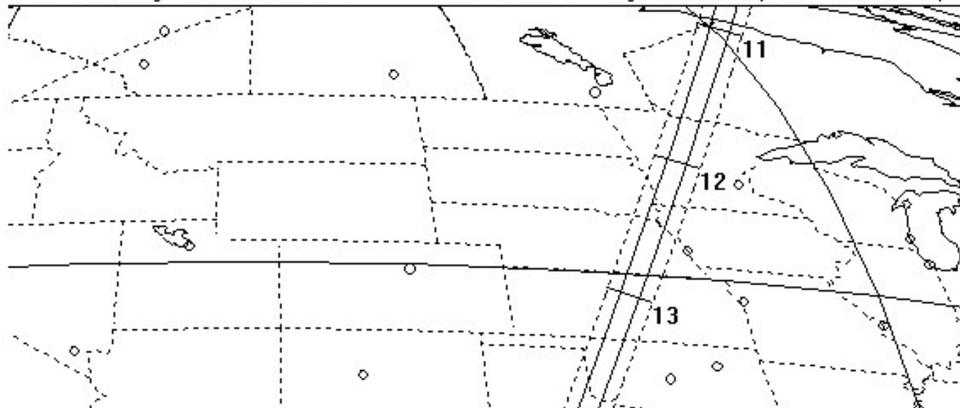
Figure 4.8. Occult prediction for the asteroid occultation of 856 Backlunda on August 15, 2004. The map projection shows the orientation of the Earth from the asteroid. Details are shown in the tabular section at the top of the chart.
