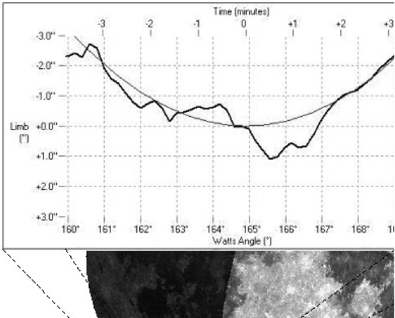
Figure 5.9 Low grazing occultation prediction for the star SAO 189348 on October 20, 2007. A lunar limb profile box is shown for the area of the graze. The target star has a 14 degree cusp angle from the southern limb.
