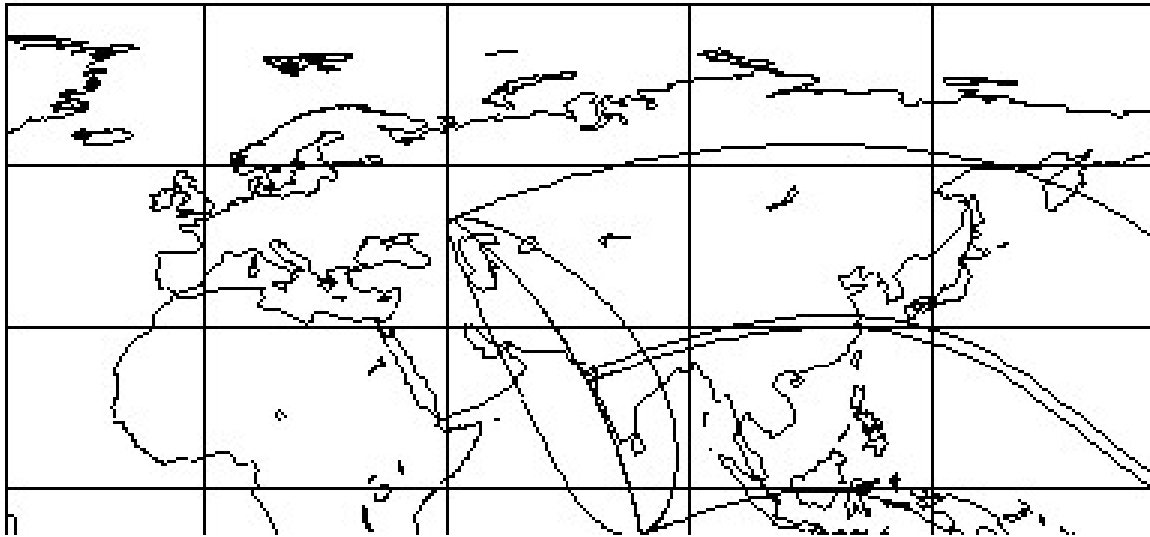
Figure 4.6. Global map projection of eclipse from July 22, 2009. The path of totality from India through China into the south Pacific Ocean is shown. The area where partial phases are visible are shown north and south of totality.
