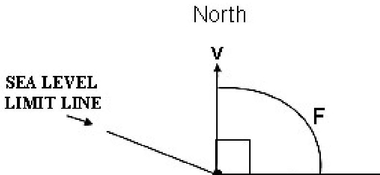
Figure 5.7b. Computing the azimuth F of the sea level limit line. F = 90 + b . A right triangle is formed from the sides AB , BI and AI .
