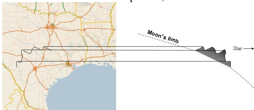
Figure 5.4. The lunar mountains and valleys are projected onto the Earth's surface. Diagram not to scale.
