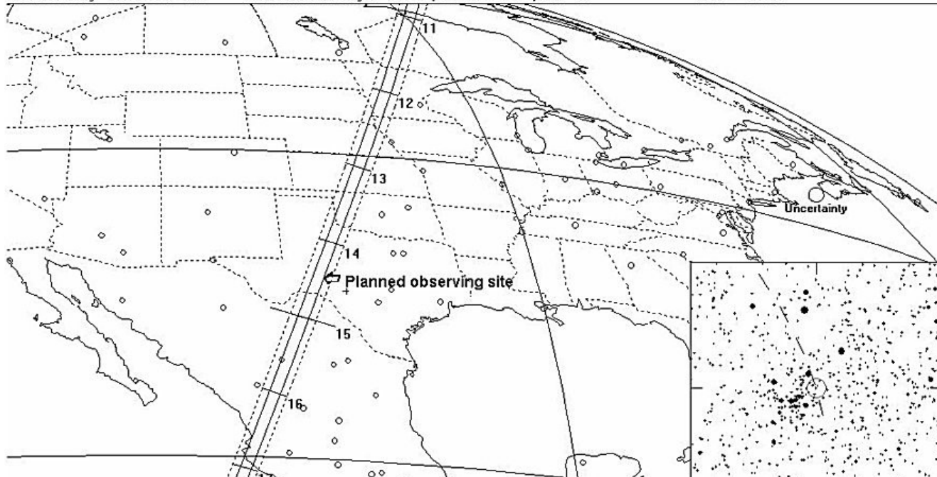
Figure 6.11. Determining your observing position from prediction updates. The pointed arrow corresponds to an event time near 4h 14m 30sec UT in central Texas. Prediction from Occult software asteroid module.
