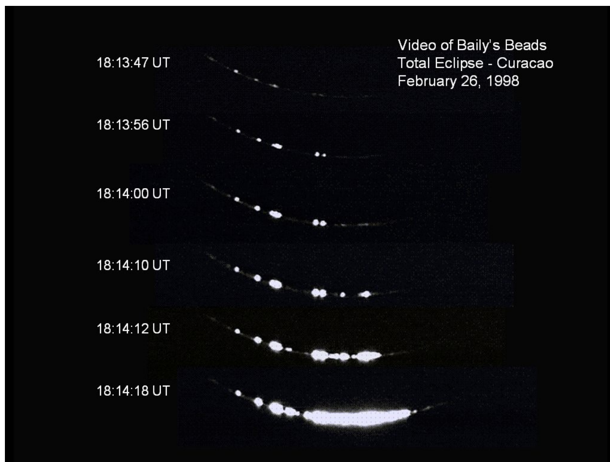
Figure 11.1. Baily's Beads. These are screen captures off a video encompassing a 31 second time interval during the central phase of the total eclipse which occurred in Curacao on February 26, 1998. Video frames by Richard Nugent.
