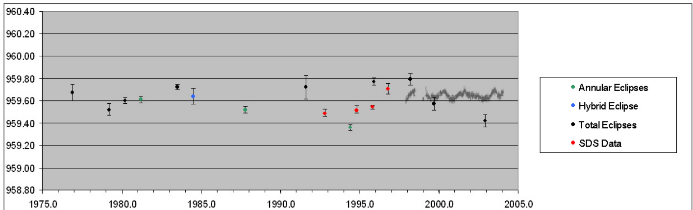
Figure 11.6. Comparison of data from several methods to measure the Sun's radius. The gray wavy line from years 1997-2004 is from the SOHO data. The vertical axis is the solar radius in arc seconds, the horizontal axis is the year the measurements were made. Diagram from Dunham, et.al., 2007.
