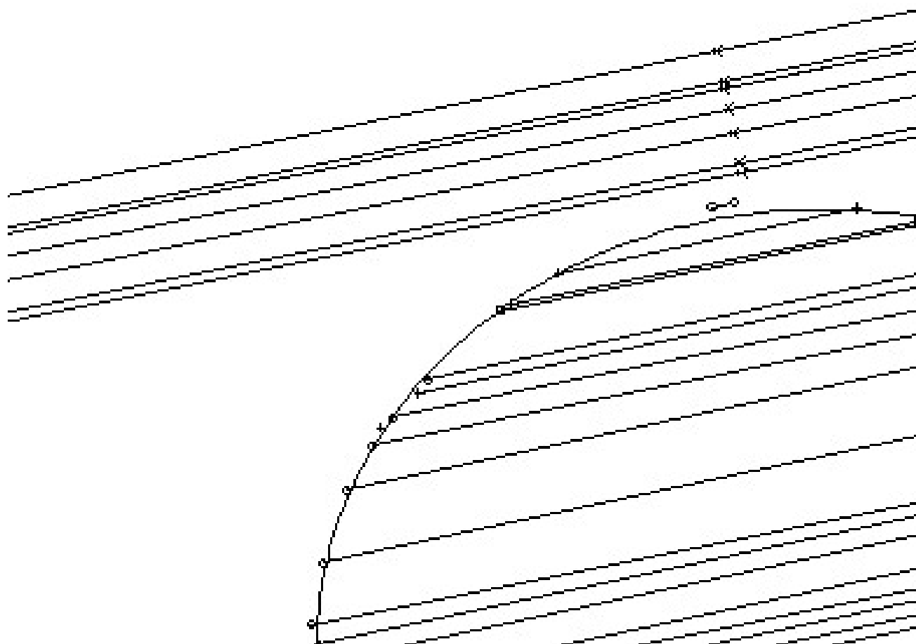
Figure 6.13. Profile of 704 Interamnia from March 23, 2003. This occultation was recorded by 54 observers in Hawaii and Japan, demonstrating international cooperation in observing occultations. Profile generated from Occult software.
