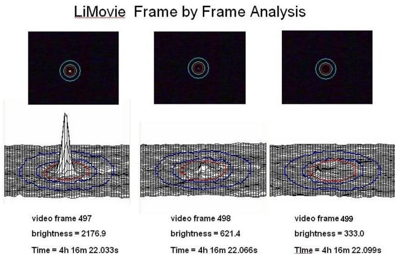
Figure 8.13. LiMovie analysis of three successive video frames. See text for explanation.
