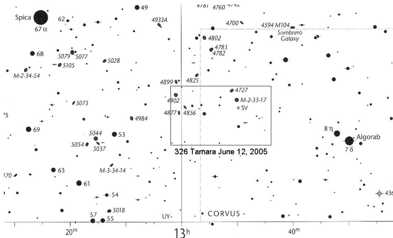
Figure 6.6. Portion of Chart 14 of Wil Tirion's Sky Atlas 2000.0 showing the region for the 326 Tamara occultation. Drawing a 3^\circ \times 5^\circ box as shown on this large full page chart greatly aids in finding the target star area fast. Sky Atlas 2000.0 © Sky Publishing Corp.
