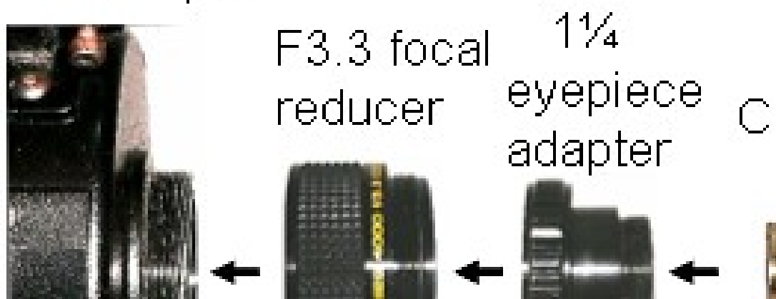
Figure G-5. Video camera attached to telescope with f3.3 focal reducer and C-mount.
