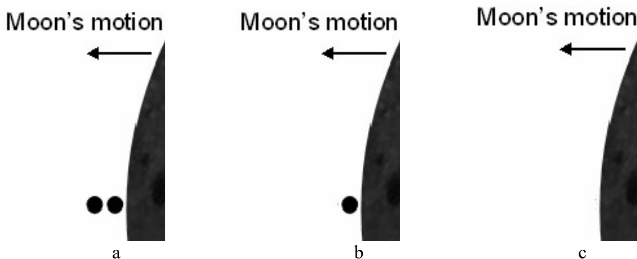
Figure 3.6 Double star geometry during an occultation. As the Moon approaches the double star (a), it first covers up one component (b) and then the second component (c). Diagrams not to scale.
