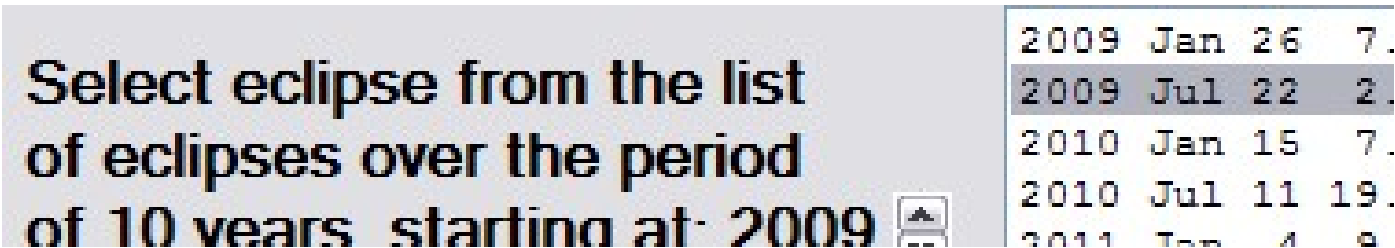
Figure 4.5. Occult Eclipses prediction window. Double click on the highlighted event (July 22, 2009 eclipse) to display a world map. See Figure 4.6 for map.
