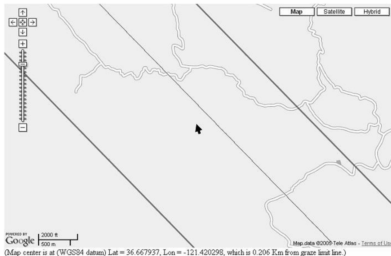
Figure 5.16. Screen shot of Google Earth Maps for the graze of ZC 1251 on May 3, 2006. The center coordinates of the map are given at the bottom and the cursor was clicked at its location to display the 0.206 km distance perpendicular to the center line.
