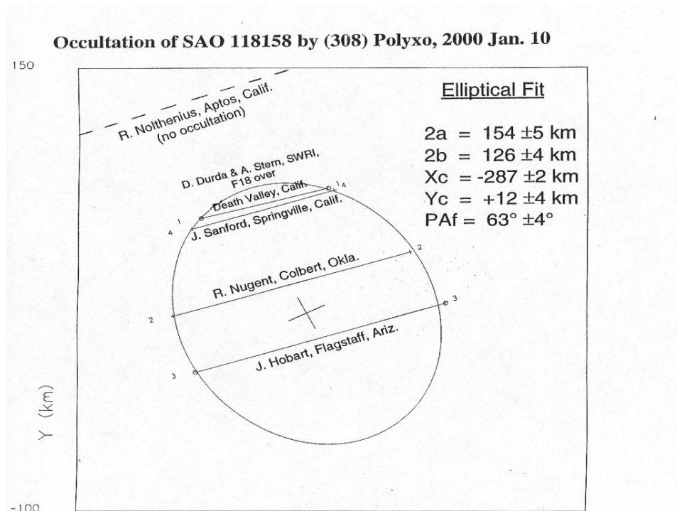
Figure 6.16. Profile of 308 Polyxo, January 10, 2000. This occultation was the first to be observed and timed from an aircraft, namely an F-18 Air Force jet over Death Valley California. Profile courtesy David Dunham.
