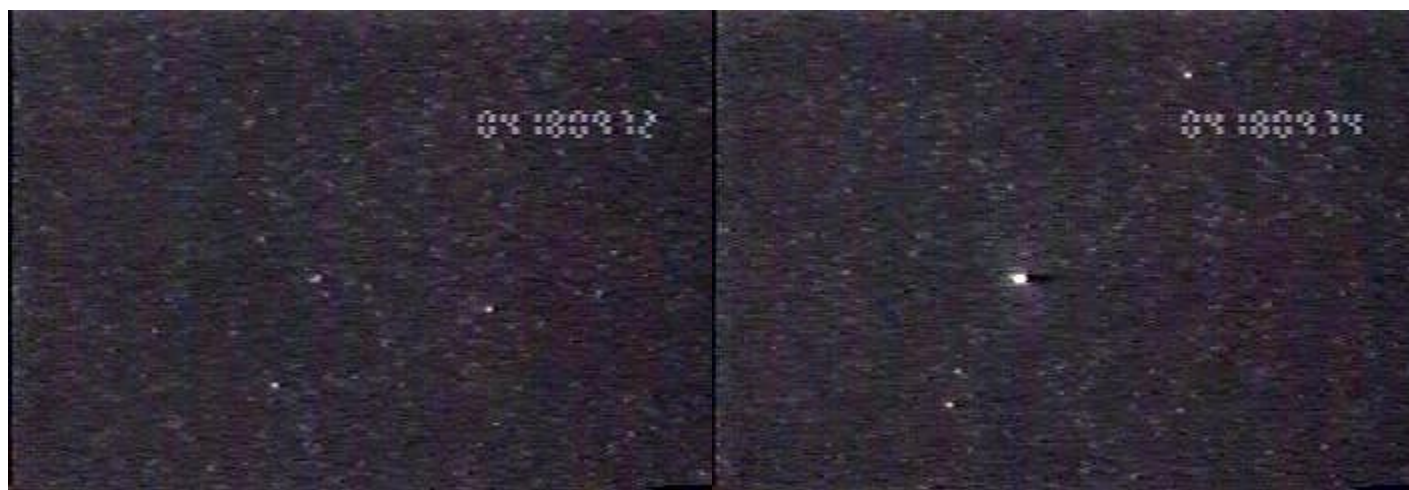
Figure 8.9. Consecutive time inserted video frames from an asteroid occultation. Time on left frame reads 4:18:09.72 = 4:18:09.733 UT (see text for explanation of decimal seconds conversion), the right frame reads 4:18:09.74 = 4:18:09.766 UT. Star has reappeared over this 0.033sec interval. The video images are quite noisy due to the use of an image intensifier. From the asteroid occultation by 129 Antigone on 9 September 2001, video by Richard Nugent and Marilyn Burke.
