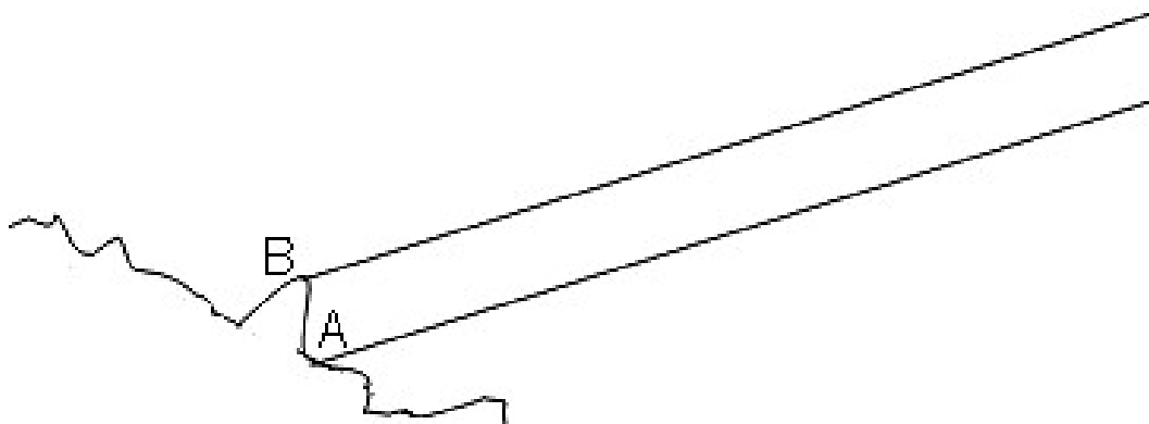
Figure 7.2. Use of elevations in occultation observations. The observer at -B- is at a higher elevation than the observer at -A-, thus he will have a slightly different view of the occultation. Diagram not to scale.
