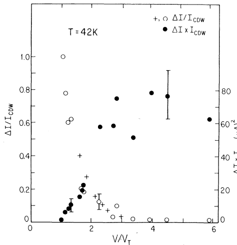
FIG. 3. \Delta I/I_{CDW} and \Delta I \times I_{CDW} vs V/V_T . Open and solid circles are constant-current pulses; crosses are constant-voltage pulses.
