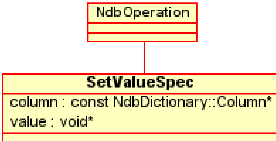
Figure 2.30 NdbOperation::SetValueSpec
