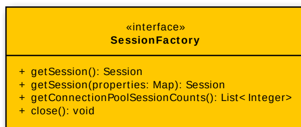
Figure 4.19 SessionFactory Class
