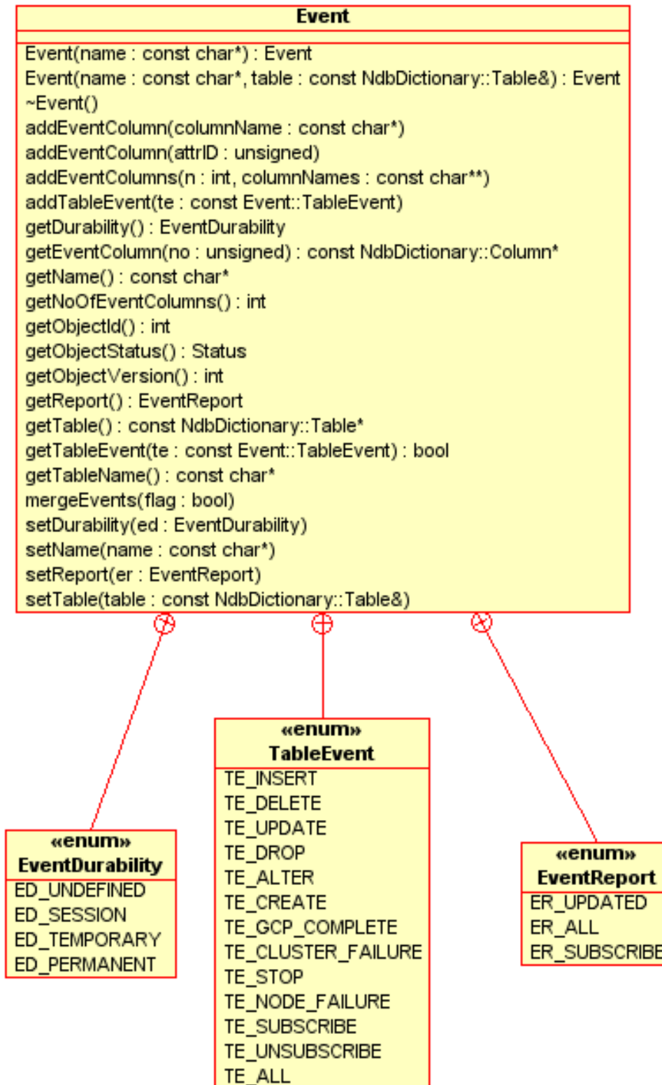
Figure 2.5 NdbDictionary::Object::Event
