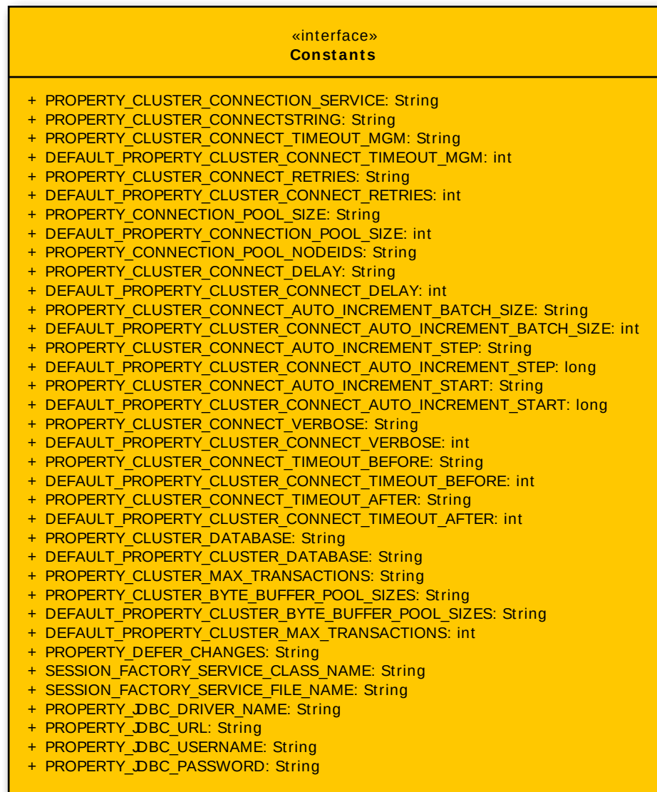
Figure 4.10 Constants Class
