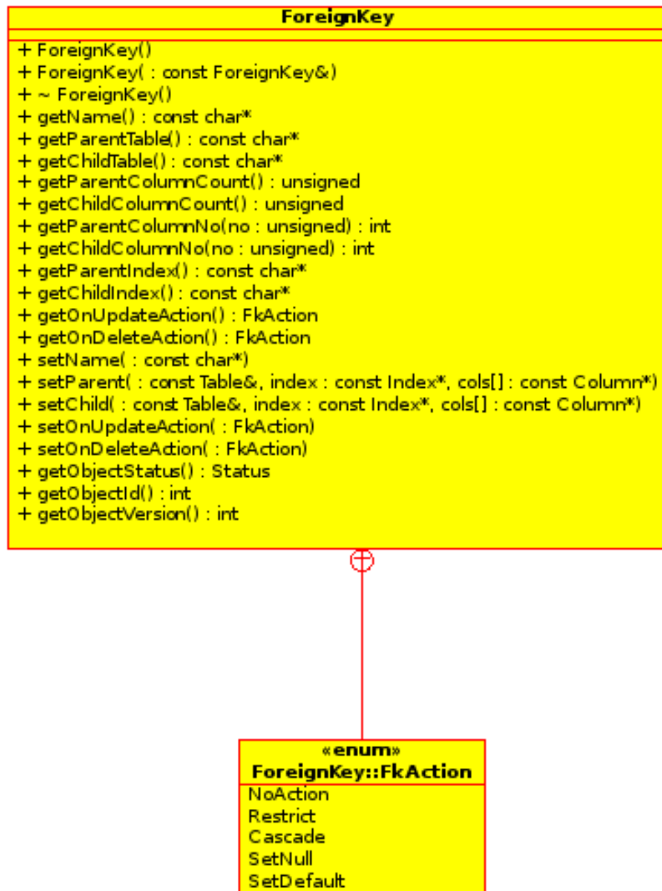
Figure 2.6 NdbDictionary::Object::ForeignKey
