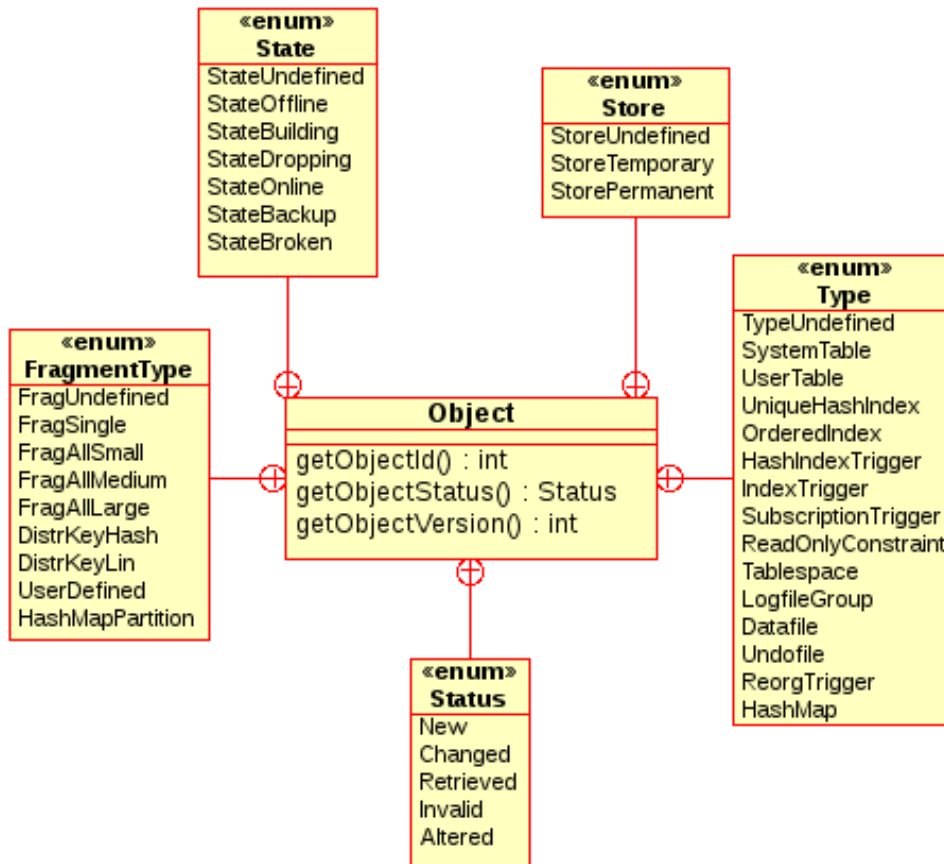
Figure 2.26 NdbDictionary::Object
