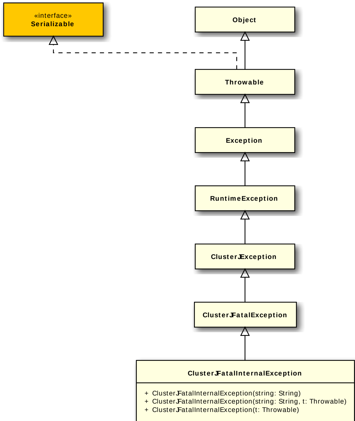
Figure 4.4 ClusterJFatalInternalException Class
