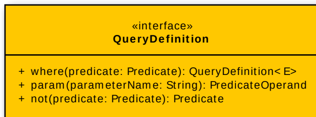
Figure 4.39 QueryDefinition Class
