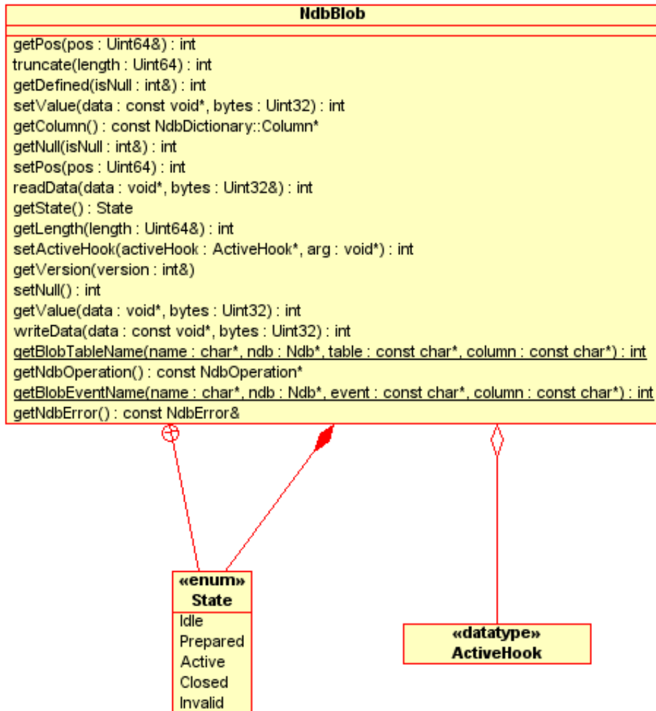
Figure 2.13 NdbBlob
