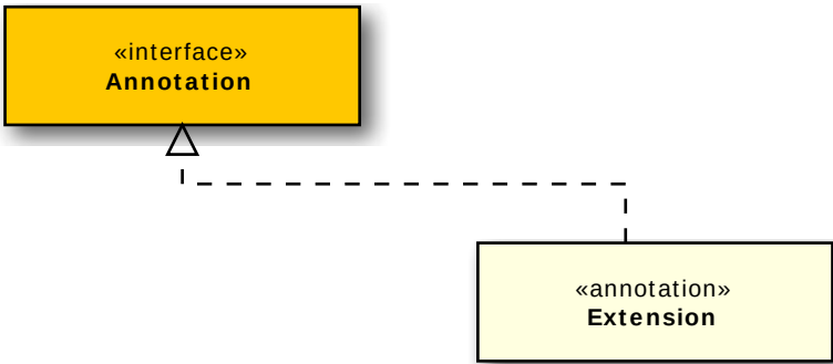
Figure 4.24 Extension Class
