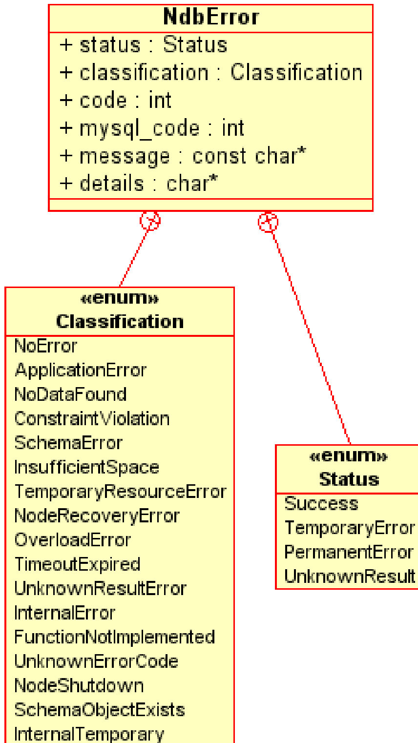
Figure 2.15 NdbError
