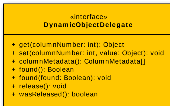
Figure 4.13 DynamicObjectDelegate Class
