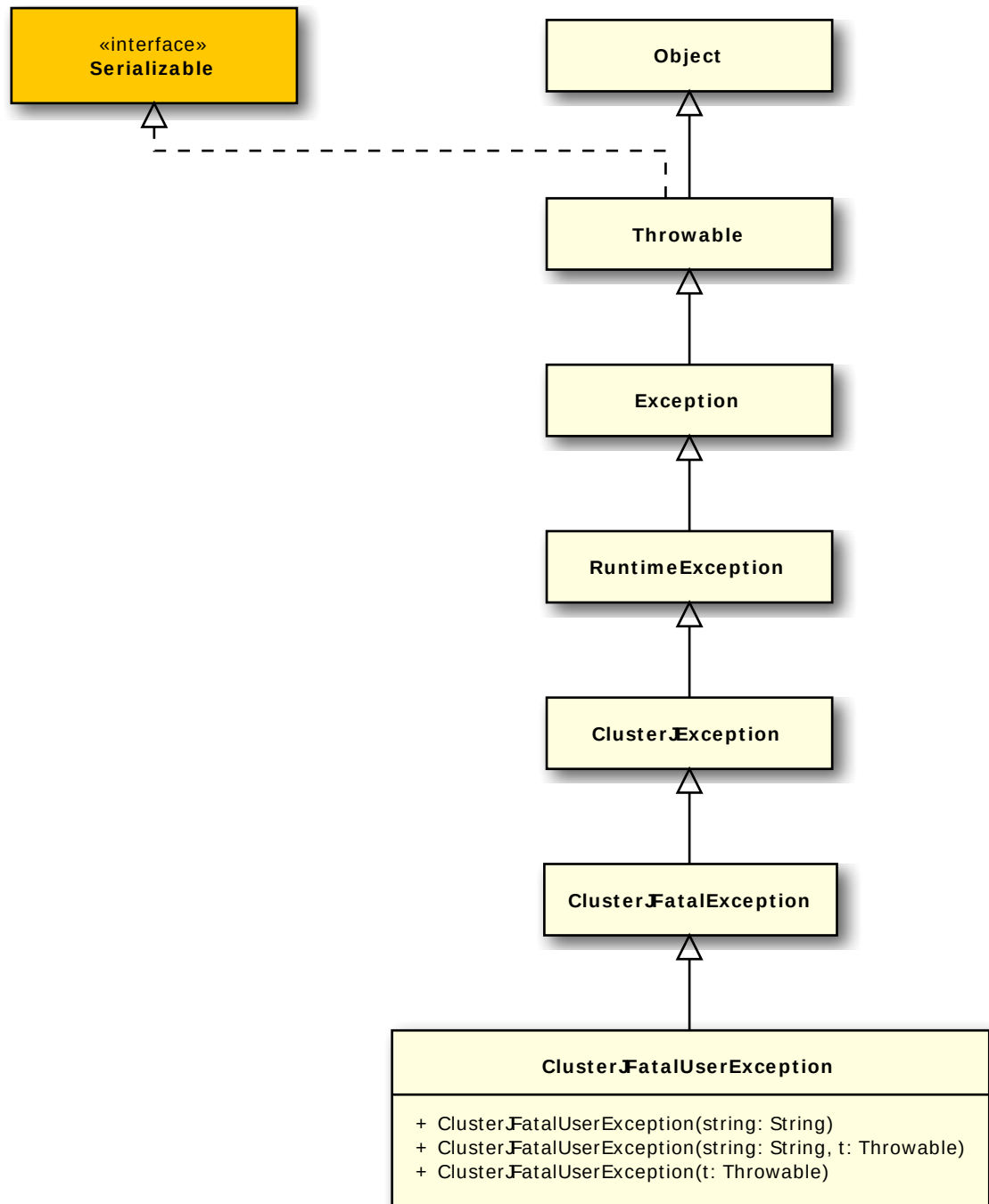
Figure 4.5 ClusterJFatalUserException Class
