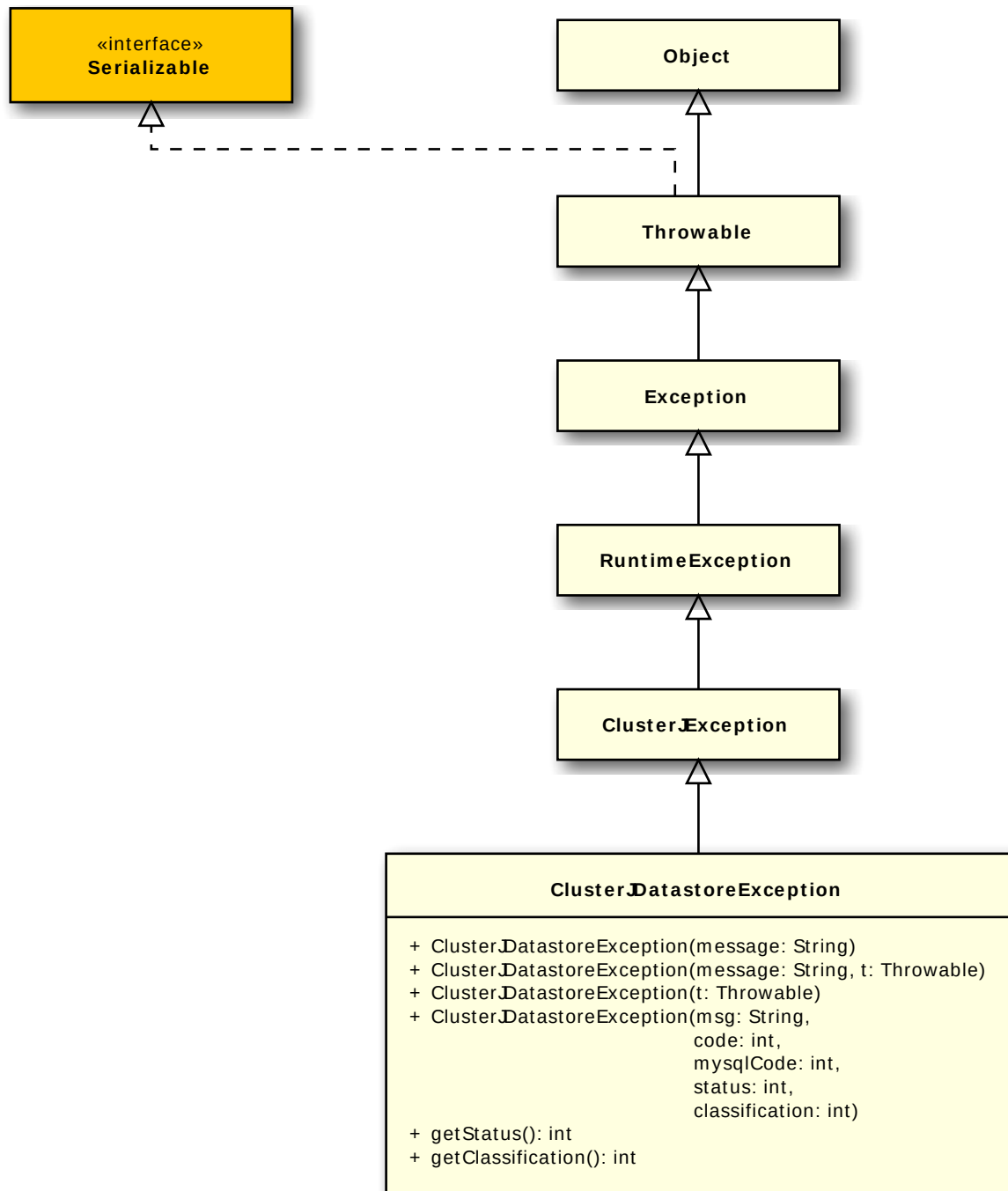
Figure 4.1 ClusterJDatastoreException Class
