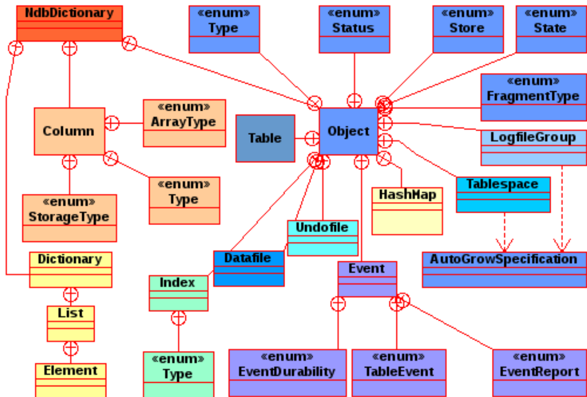
Figure 2.14 NdbDictionary subclasses
