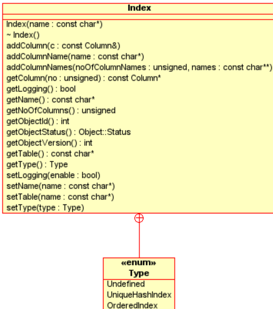
Figure 2.9 NdbDictionary::Object::Index
