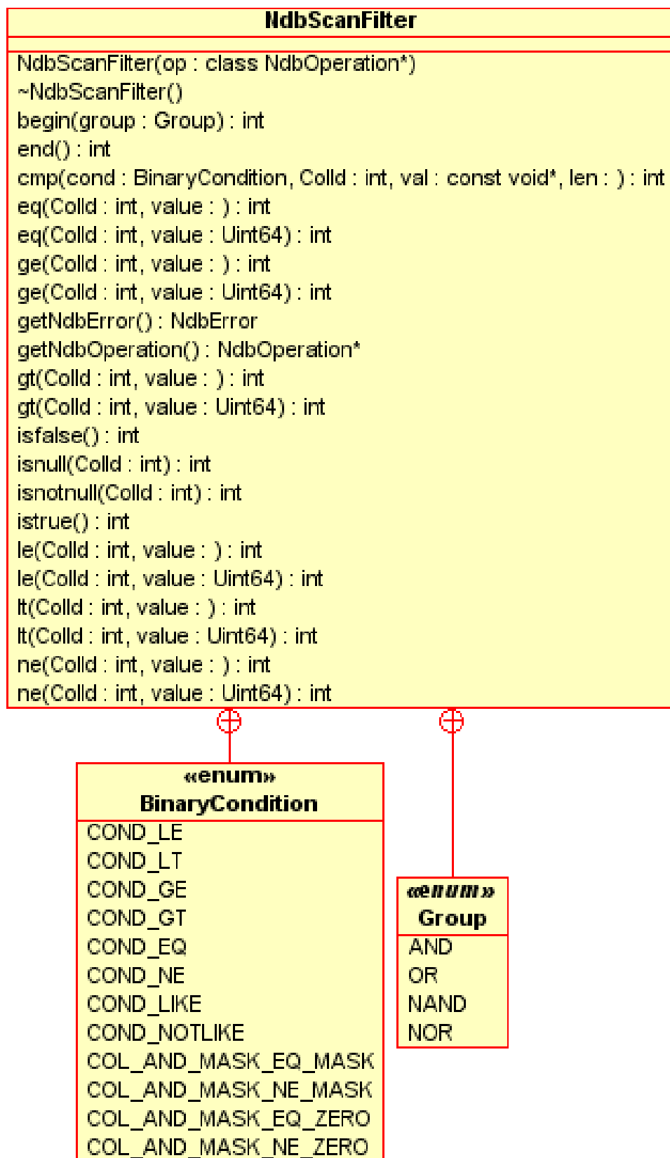
Figure 2.23 NdbScanFilter
