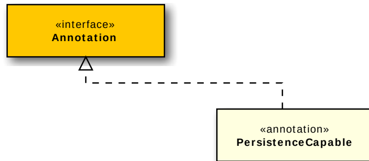
Figure 4.32 PersistenceCapable Class
