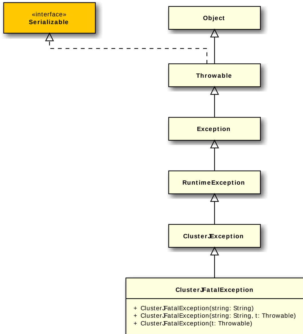
Figure 4.3 ClusterJFatalException Class
