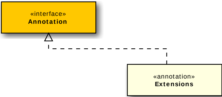
Figure 4.25 Extensions Class
