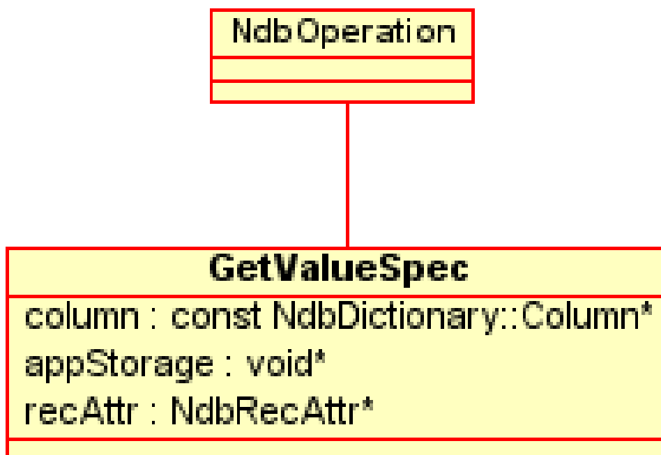
Figure 2.7 NdbOperation::GetValueSpec
