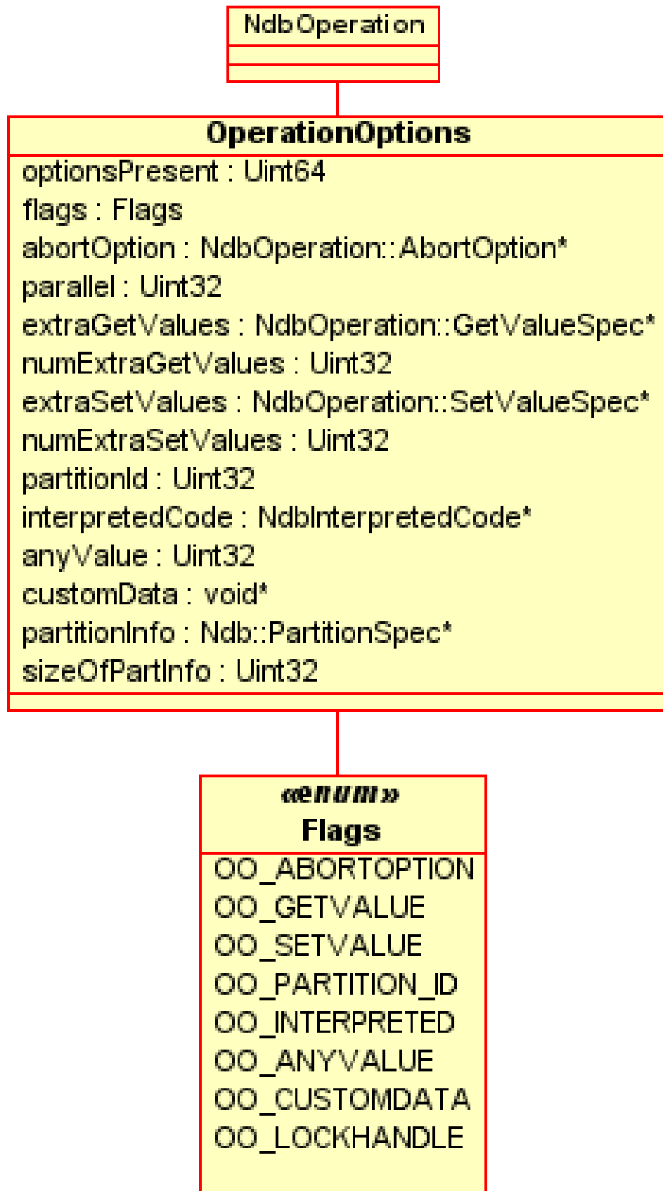
Figure 2.27 NdbOperation::OperationOptions
