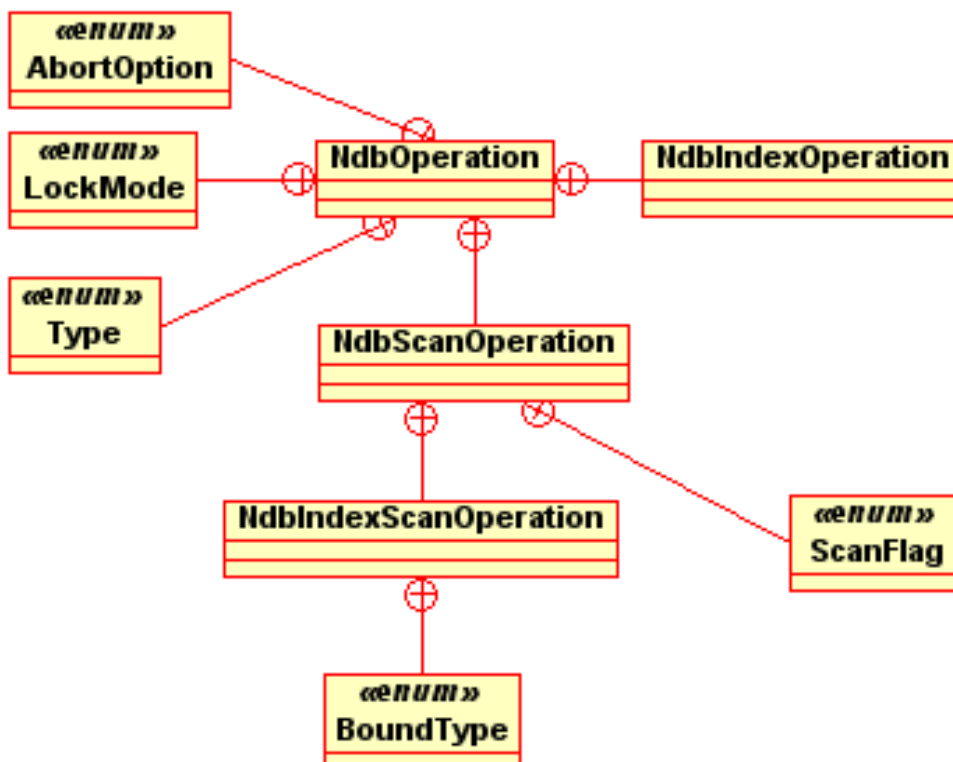
Figure 2.20 NdbOperation subclasses
