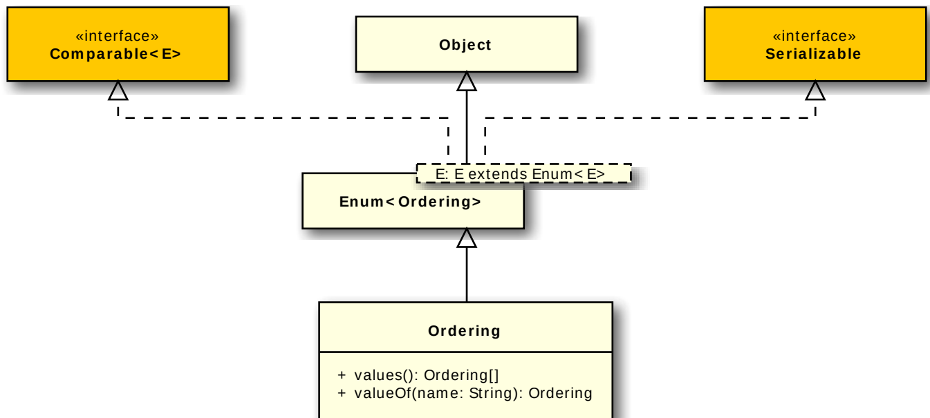
Figure 4.16 Query.Ordering Class
