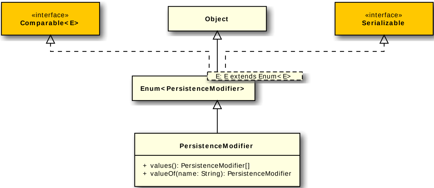
Figure 4.33 PersistenceModifier Class
