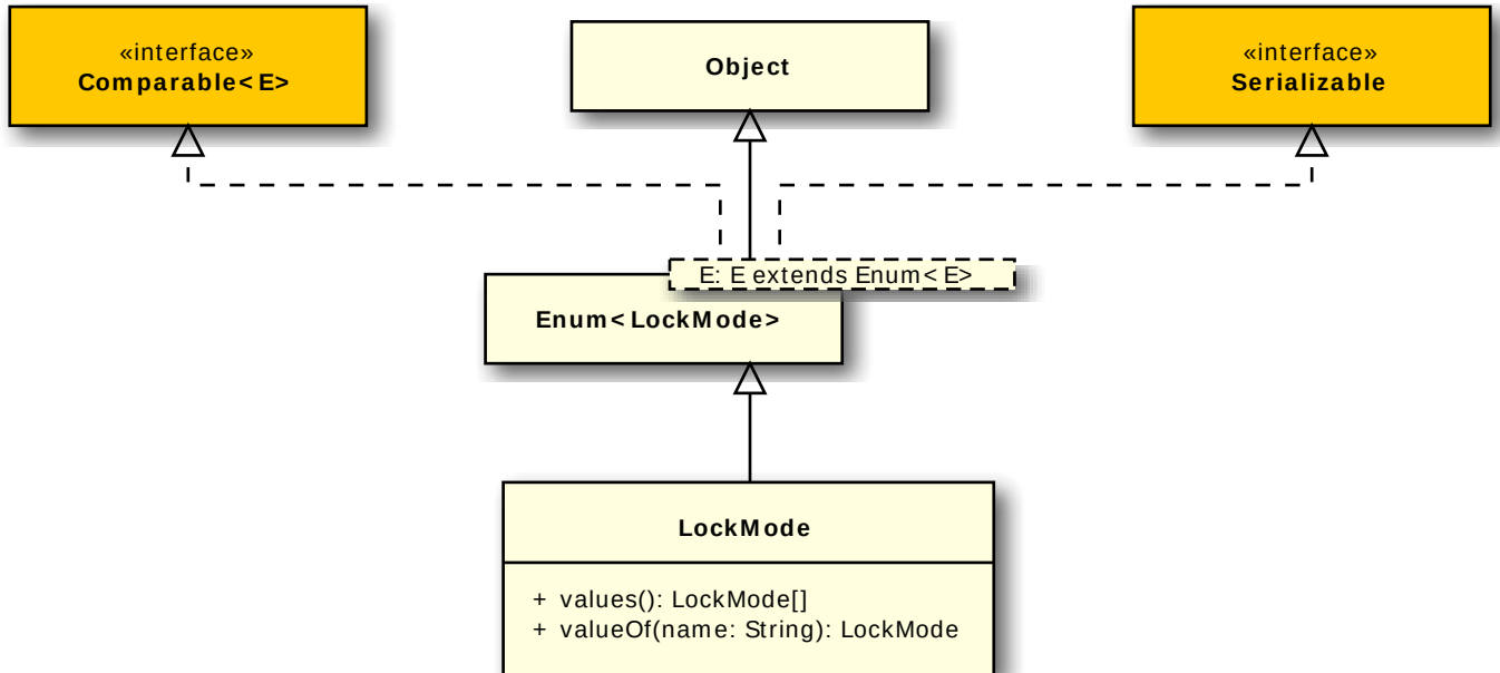
Figure 4.14 LockMode Class
