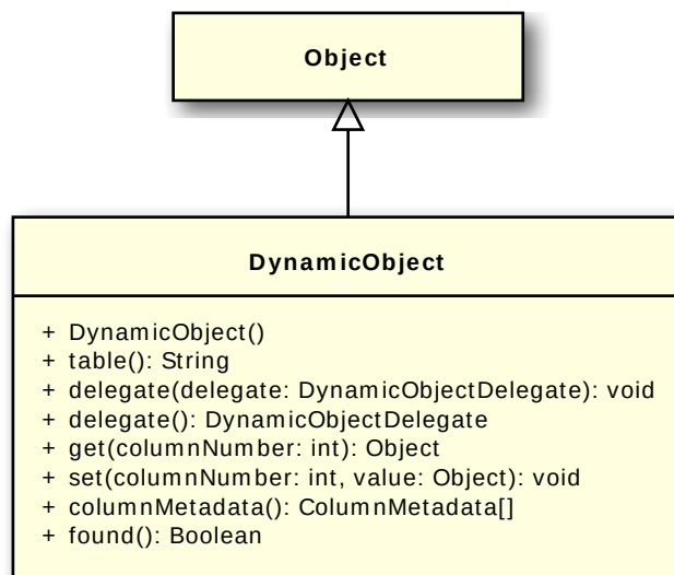
Figure 4.12 DynamicObject Class
