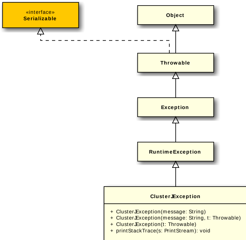
Figure 4.2 ClusterJException Class
