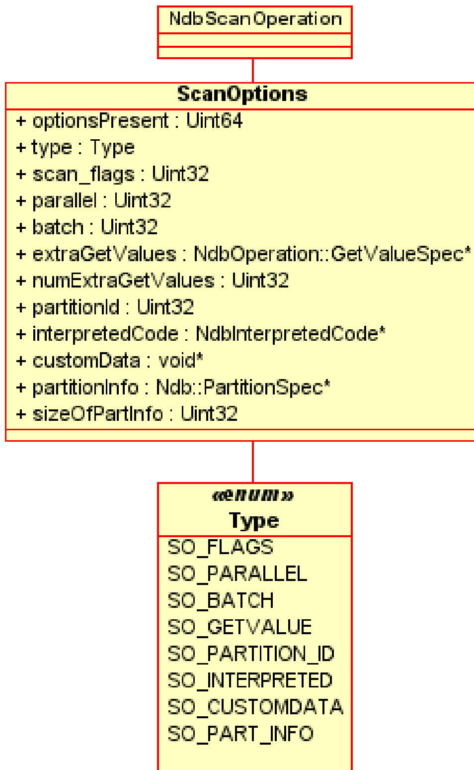
Figure 2.29 NdbScanOperation::ScanOptions
