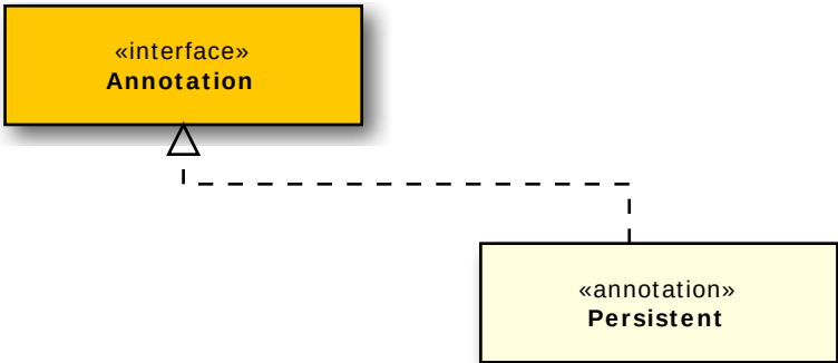
Figure 4.34 Persistent Class
