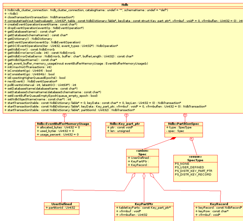
Figure 2.11 Ndb
