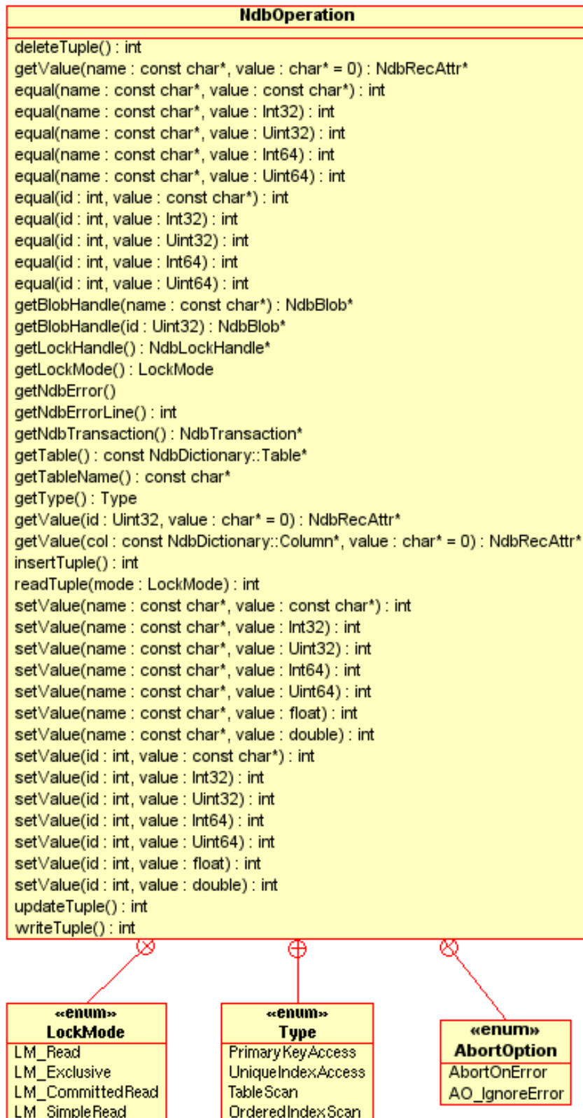
Figure 2.21 NdbOperation
