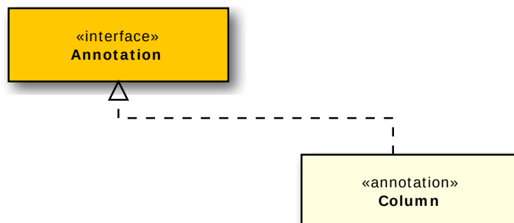
Figure 4.22 Column Class
