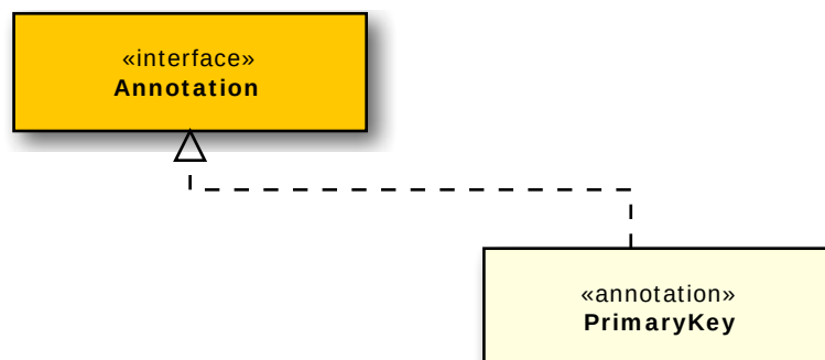
Figure 4.35 PrimaryKey Class
