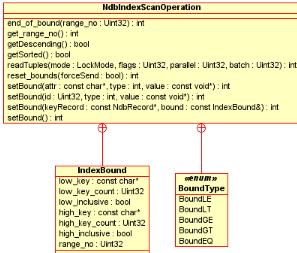
Figure 2.18 NdbIndexScanOperation
