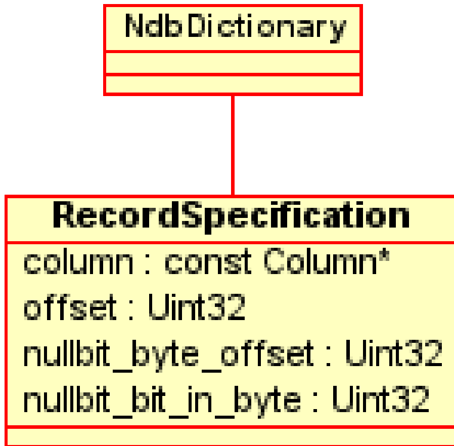
Figure 2.28 NdbDictionary::RecordSpecification
