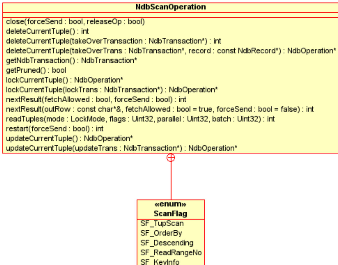
Figure 2.24 NdbScanOperation
