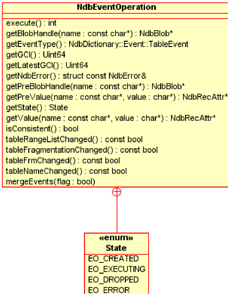
Figure 2.16 NdbEventOperation
