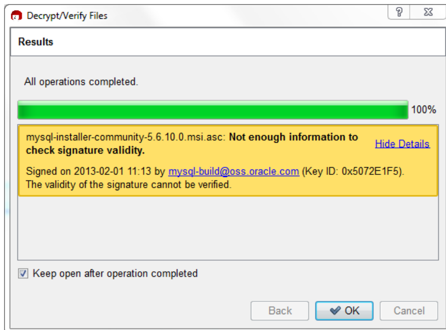
Figure 2.5 The Decrypt/Verify Results: Good
